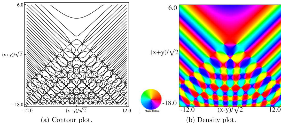
Figure 36.3.19: Phase of hyperbolic umbilic canonical integral \text{ph } \Psi^{(H)}(x, y, 1) .
