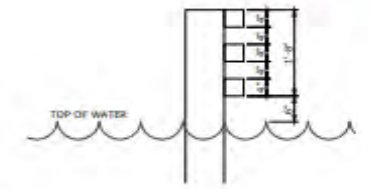
4 WAVE ATTENUATOR - SECTION SCALE: 3/4" = 1'-0" X16.0
