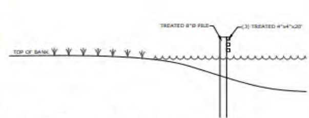
3 WAVE ATTENUATOR - SECTION SCALE: 1/4" = 1'-0" X16.0
