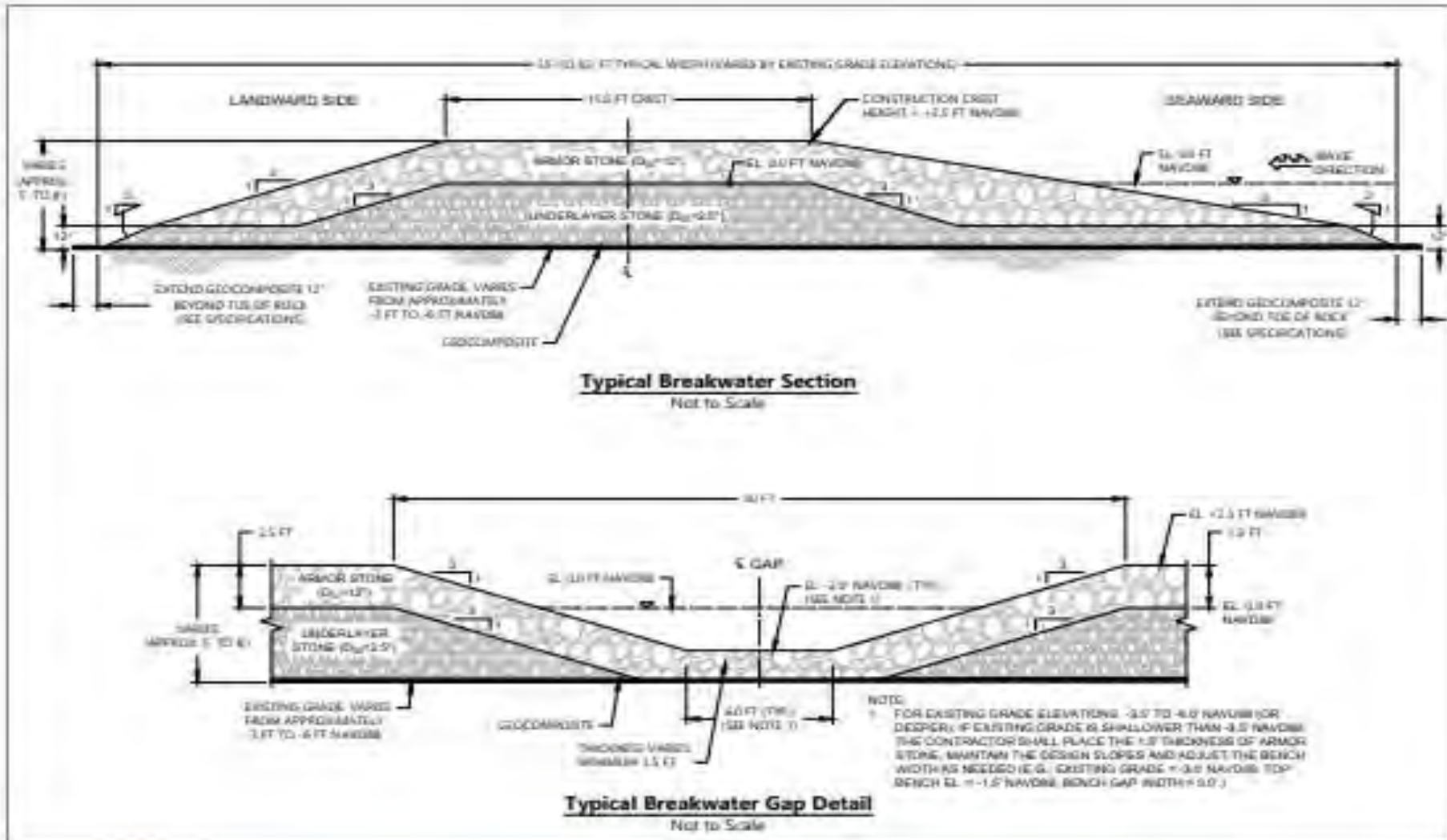
Figure 6 Typical Phase 6 Living Shoreline Breakwater Section and Detail
