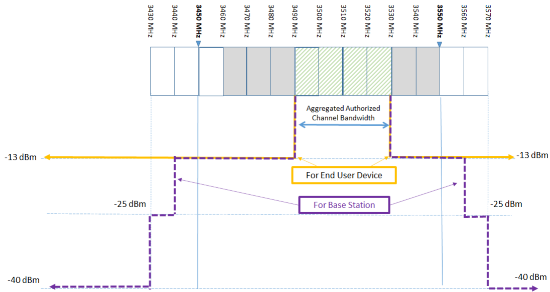
Figure 2: Emissions Mask
