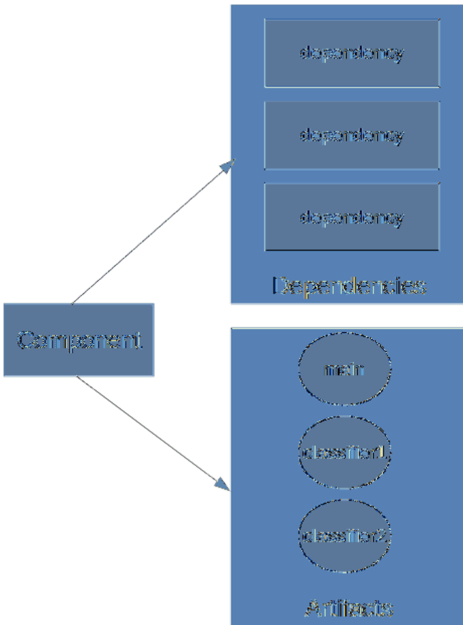
Figure 20. The Maven component model
