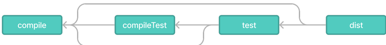
Figure 22. Simple Task Graph
