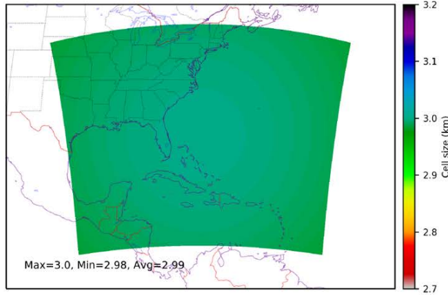
Extended Schmidt gnomonic grid
