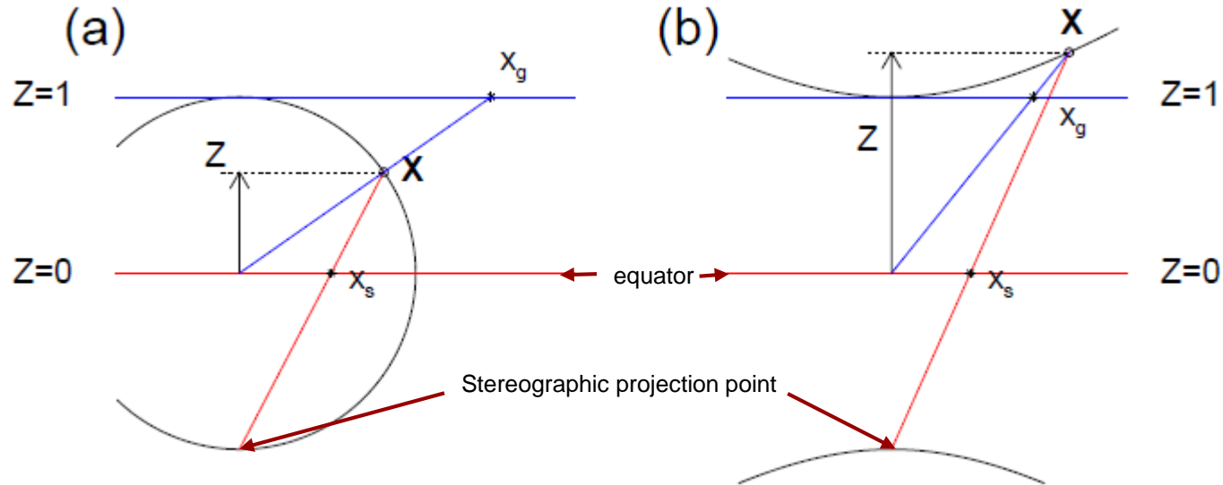
Gnomonic and stereographic projections illustrated for a true sphere of curvature K=+1
