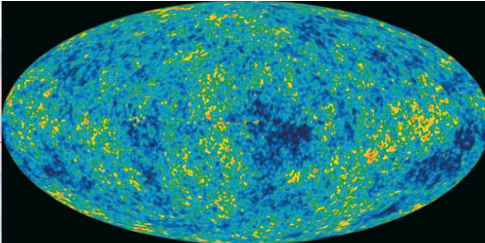
In 1992, NASA's COBE satellite confirmed for the first time that the temperature of the Cosmic Microwave Background (CMB) was not uniform over the sky. The COBE measurements indicated that over angular scales larger than 10^\circ , the temperature of the CMB varies by about one part in 100 000 from the average value of 2.73K. In 2003, COBE's successor WMAP was able to improve dramatically the map's clarity and sharpness; the image shows the tiny irregularities in the temperature of the CMB across the sky, as mapped by WMAP. (NASA)
