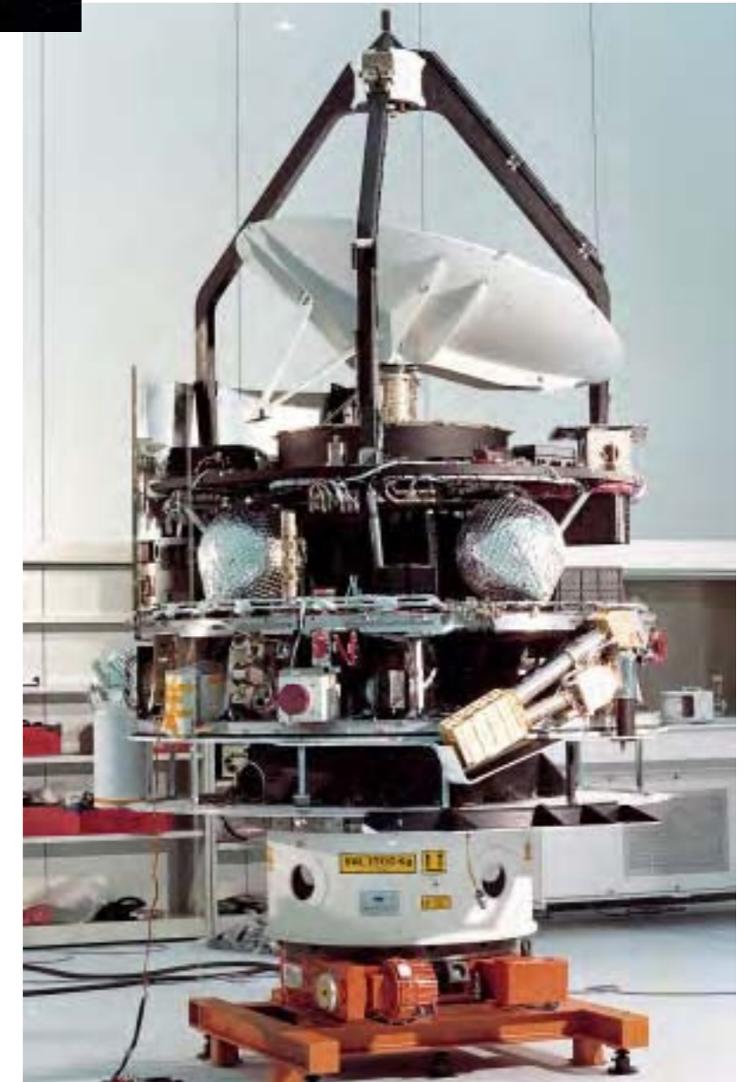
Giotto with the cylindrical solar cell array removed. Shown on the payload platform are (from left to right) the Halley Multicolour Camera (HMC), the electronics box of the Dust Impact Detection System (DIDS), the Rème Plasma Analyser (RPA) with its red cover on, and the dust mass spectrometer (PIA). Seen on the upper platform are two of the four hydrazine fuel tanks for attitude and orbit control.
