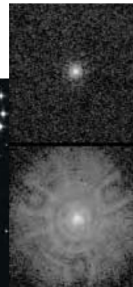
FOC images of a single star before (bottom) and after COSTAR. The halo of poorly focused light is completely rectified by COSTAR.
