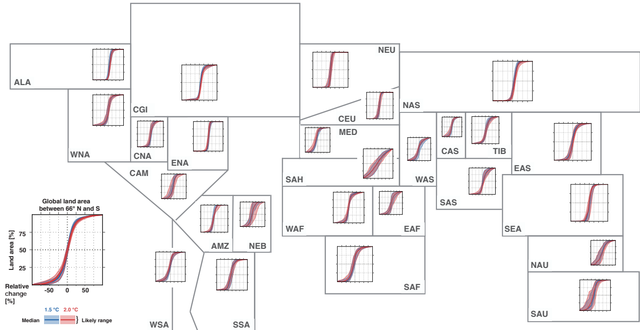
Figure 8. Same as Fig. 2 but for total annual runoff. Changes are given relative to the 1986–2005 reference period.
