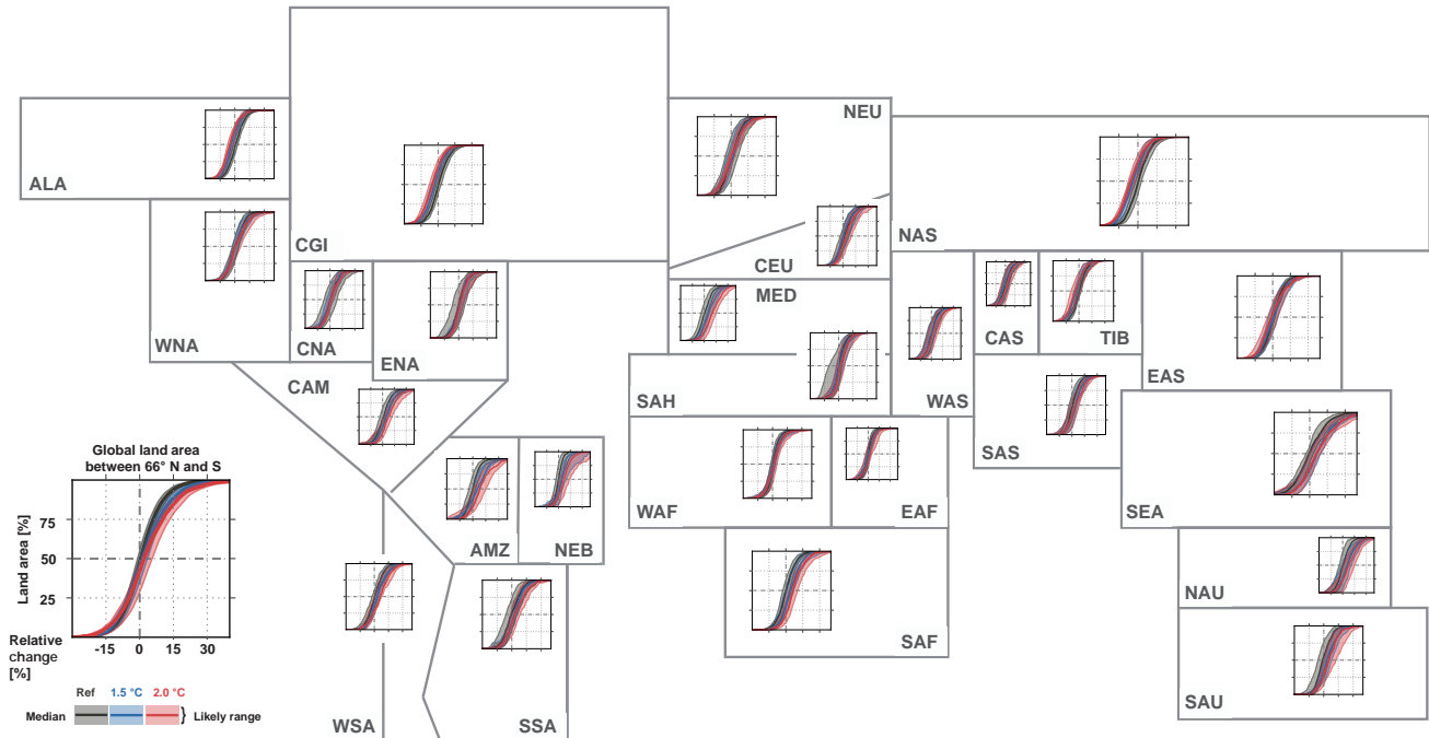
Figure 6. Same as Fig. 2 but for CDD. Changes are given relative to the 1986–2005 reference period.
