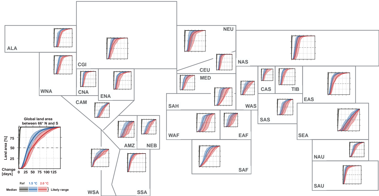
Figure 3. Same as Fig. 2, but for WSDI in days.
