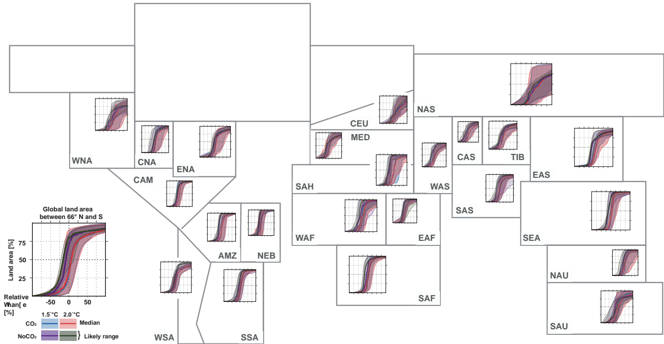
Figure 12. Same as Fig. 9 but for changes in rice yields.
