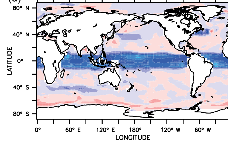
RCP8.5_AOA_T
