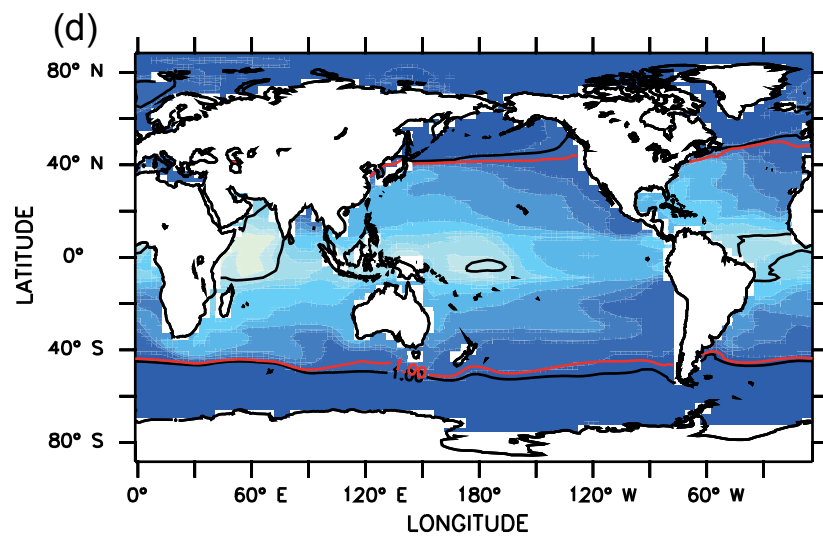
RCP8.5_AOA_T
