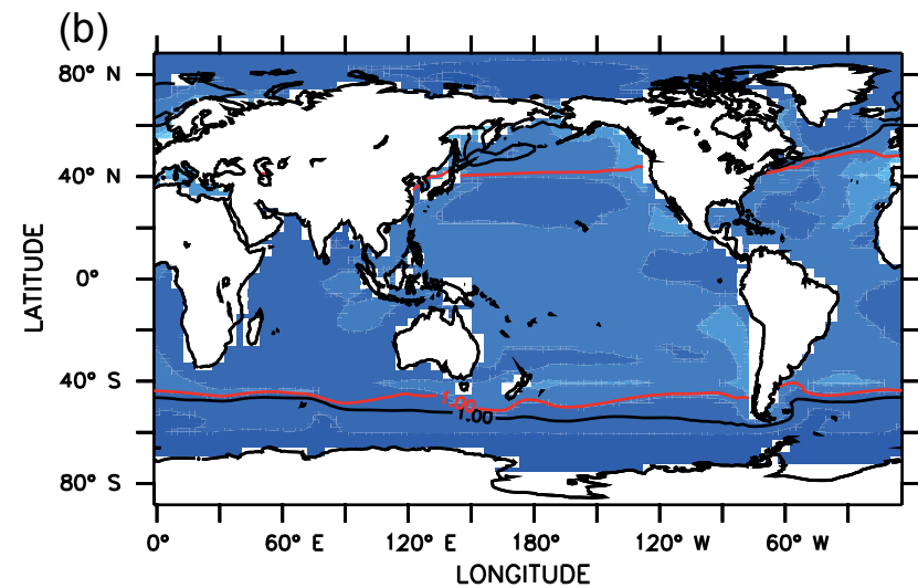
RCP8.5_AOA_SP
