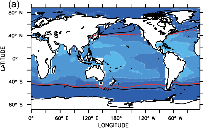
RCP8.5_AOA_G
