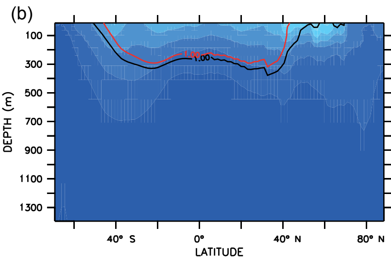
RCP8.5_AOA_SP
