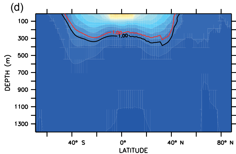
RCP8.5_AOA_T
