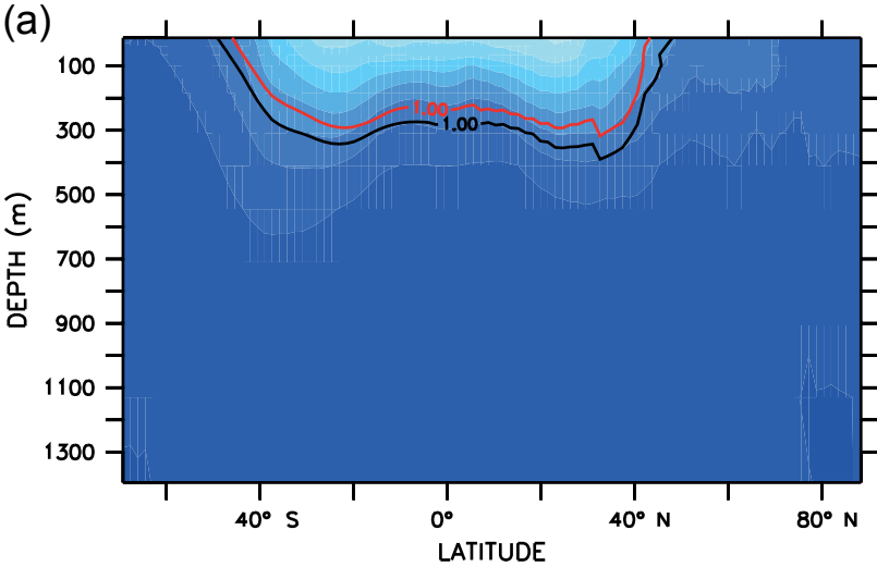
RCP8.5_AOA_G
