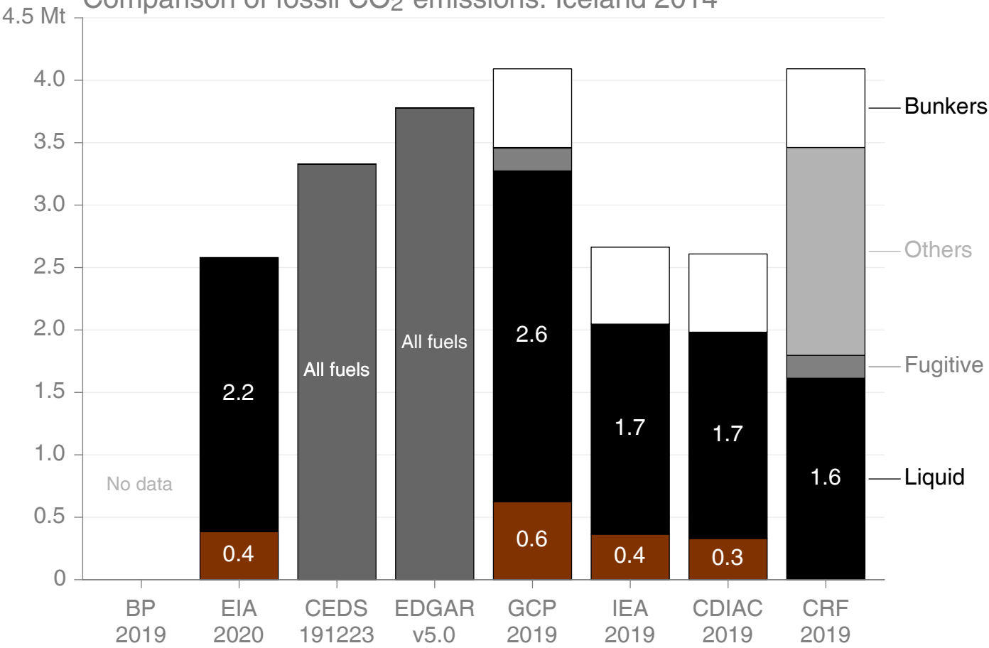
Comparison of fossil CO 2 emissions: Iceland 2014
