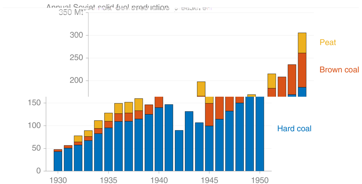
Figure SI-4: Solid fuel production in the Soviet Union (Etemad and Luciani, 1991).
