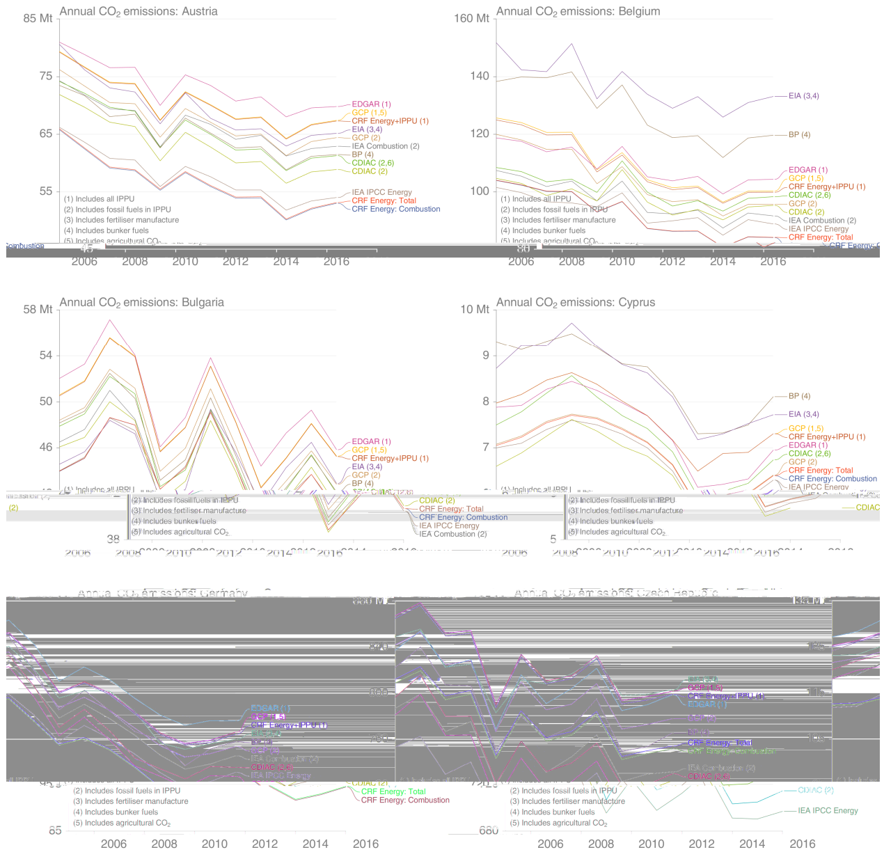
Figure SI-16: Annual CO 2 emissions for EU28 countries from various sources. For details see text.
