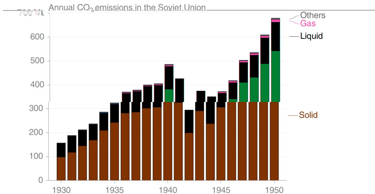
Figure SI-2: Emissions of CO 2 in the Soviet Union, 1930–1950 (Gilfillan et al., 2019).
