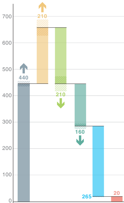
Cumulative changes 1850–2019
