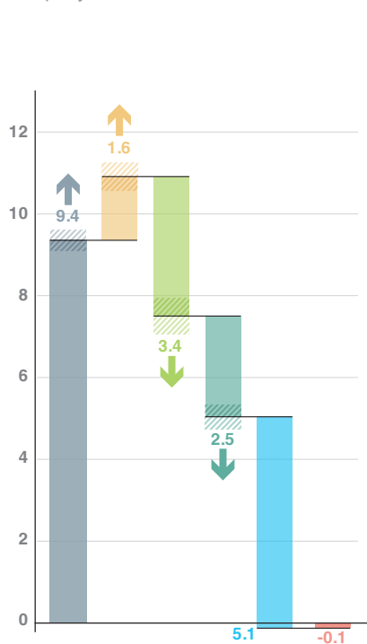
Mean fluxes 2010–2019
