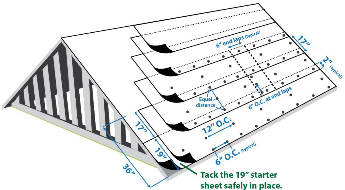
Figure 4. Installation of 19 in. starter course
