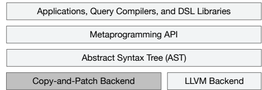
Fig. 6. Copy-and-Patch can be used by metaprogramming systems to speed up their interpreters past LLVM -O0 . And it can be combined with LLVM to let the user request higher optimization levels when the increased performance can amortize the orders of magnitude higher compilation cost.
