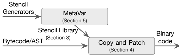
Fig. 4. The copy-and-patch system compiles a high-level language AST or a bytecode sequence to binary code. It consists of the MetaVar compiler, which compiles stencil generators to binary stencils, and the Copy-and-Patch code generator, which generates the executable code for an AST or a bytecode sequence by copying and patching stencils.
