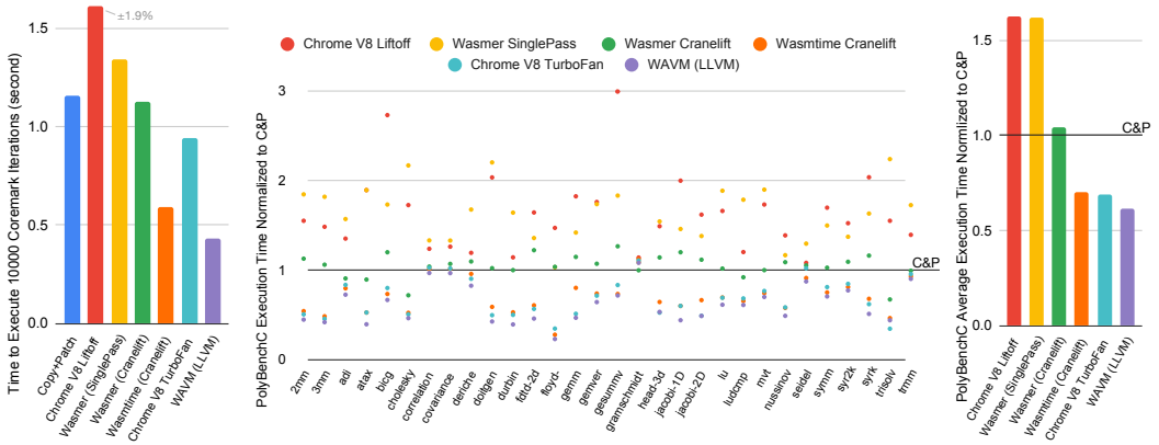
Fig. 20. WebAssembly exec time, Coremark. Fig. 21. WebAssembly normalized execution time on each of the 30 PolyBenchC benchmarks, normalized to copy-and-patch. Fig. 22. Average of Figure 21.
