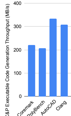
Fig. 19. Throughput of machine code generated by copy-and-patch (MB/s).
