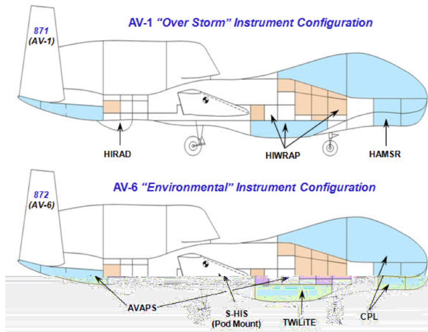
Figure 1-2 shows the baseline instrument configurations on the two GHs for 2014.
