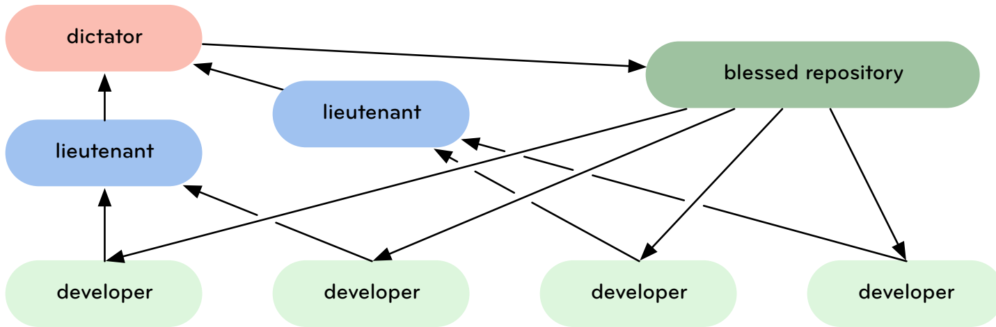
FIG. 1 Approved features gradually make their way up the ladder
