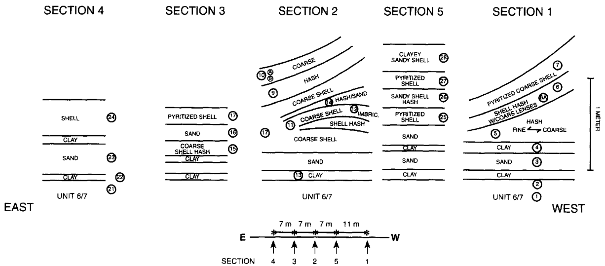
Fig. 3. Schematic cross-section of exposures of the bird layers from which invertebrate samples (IS) for taphonomic analysis were collected. Circled numbers refer to IS numbers; only 8 of the 22 samples taken are discussed here. Cormorant bones and partial skeletons were found throughout all of the layers illustrated here except units 6/7.
