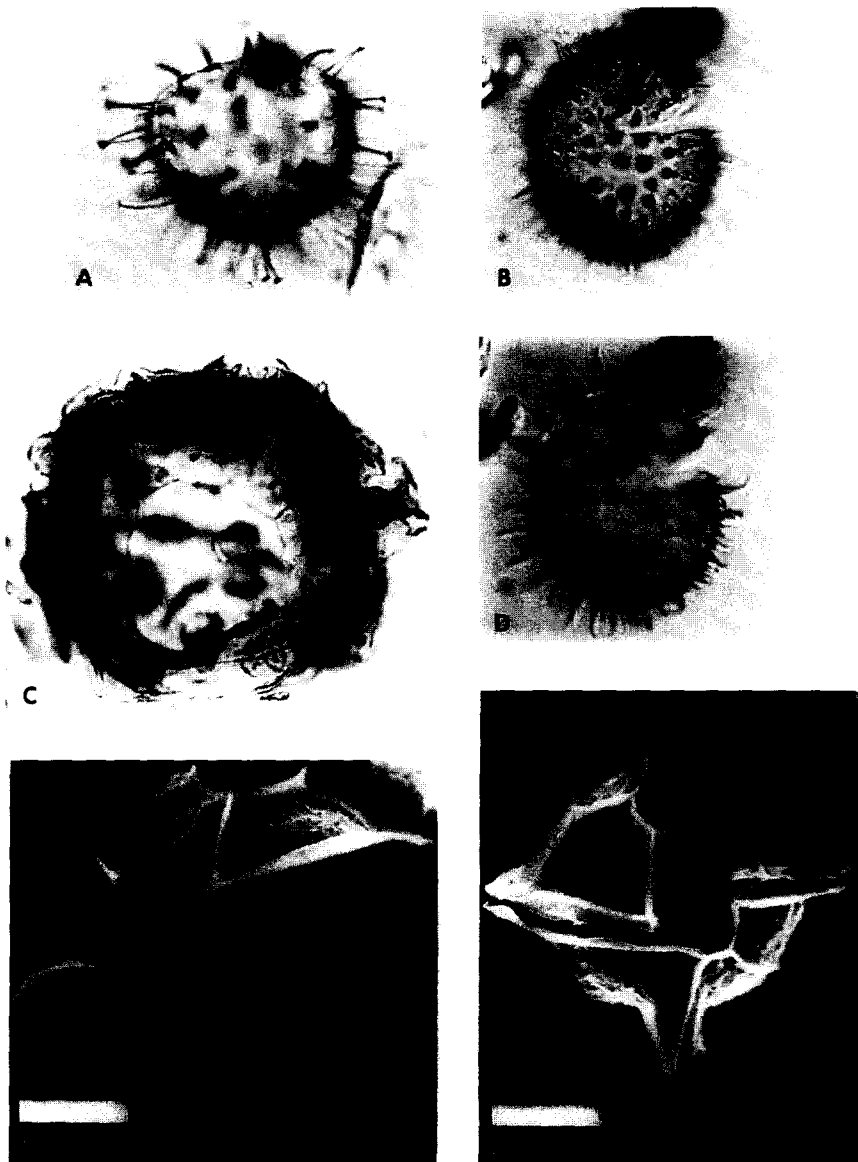
Fig. 10. Fossil dinocysts (a–d) recovered from the “Pinecrest Sand” at Richardson Road Shell Pit and thecate specimens (e–f) of Pyrodinium bahamense . (a) Polysphaeridium zoharyi (Rossignol) Bujak et al. Slide 3 (+45 \mu\text{m} ); coordinates 121.5 \times 12.9; magnification 400 \times ; (b,d) Lingulodinium machaerophorum (Deflandre and Cookson) Wall. Slide 2 (+45 \mu\text{m} ); coordinates 110.1 \times 4.9; magnification 400 \times ; (c) Tuberculodinium vancampoae (Rossignol) Wall. Slide 2 (+45 \mu\text{m} ); coordinates 102.9 \times 10.0; magnification 400 \times ; (e) Pyrodinium bahamense var. compressum (Bohm) Steidinger, Tester and Taylor 1980; scale bar = 20 \mu\text{m} ; (f) Pyrodinium bahamense var. bahamense Steidinger, Tester and Taylor 1980; scale bar = 20 \mu\text{m} (photos e and f courtesy of K. Steidinger, Florida Marine Research Institute).
