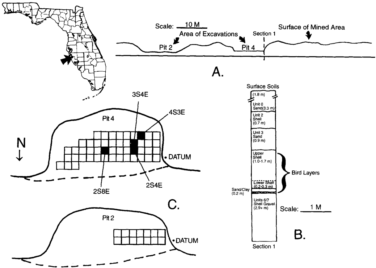
Fig. 1. Location and stratigraphy of the fossil deposits at Richardson Road Shell Pit, Sarasota County, Florida. A. Map with arrow pointing to location of the site, and cross-section of the south wall of the canal in which the site was discovered showing the extent of the deposits in the upper "Pinecrest Sand". The vertical dashed line locates the stratigraphic section shown in B and corresponds with section 1 in Fig. 3. B. Stratigraphic section of the units exposed in the upper Pinecrest "Sand" showing the location of the bird layers. C. Plan views extracted from the south wall of the canal in A of Pits 2 and 4 to show the grids and excavated 1 \times 1 m squares. The grid outline for Pit 4 is repeated in Fig. 5 to illustrate variations in bone density throughout the excavated squares. The shaded squares are labeled by location from the datum and correspond with peak concentrations of bone as shown in Fig. 5.
