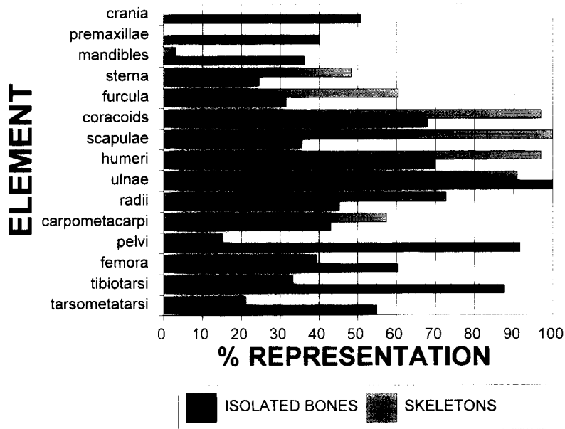
Fig. 7. Percent representation of isolated skeletal elements from the total minimum number of individuals (MNI, solid bars; 225 individuals based on ulnae) and bones in 83 associated skeletons (hatched bars; MNI=33 based on scapulae) from the excavated grids (Pits 2 and 4) at Richardson Road Shell Pit, Sarasota County, Florida. A clear distinction is apparent in the associated skeletons, which are biased towards wing elements, versus the isolated bones that show high numbers of wing and leg elements. Vertebrae were not included in these analyses.
