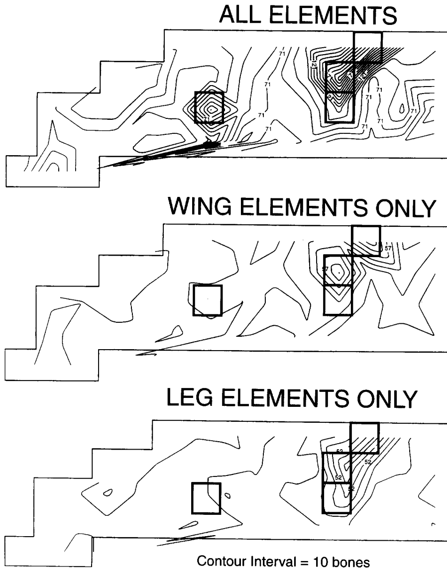
Fig. 5. Plan views of the grid in Pit 4 (see Fig. 1) indicating relative density of bone using contour intervals of 10 from all three of the bird layers for the total sample (top, base contour = 7), wing elements only (coracoid, humerus and ulna; middle, base contour = 17) and leg elements only (femur, tibiotarsus and tarsometatarsus; bottom, base contour = 12). Peak concentrations (highest contours) occur in squares 3S4E and 4S3E (see Fig. 1) outlined in each diagram.
