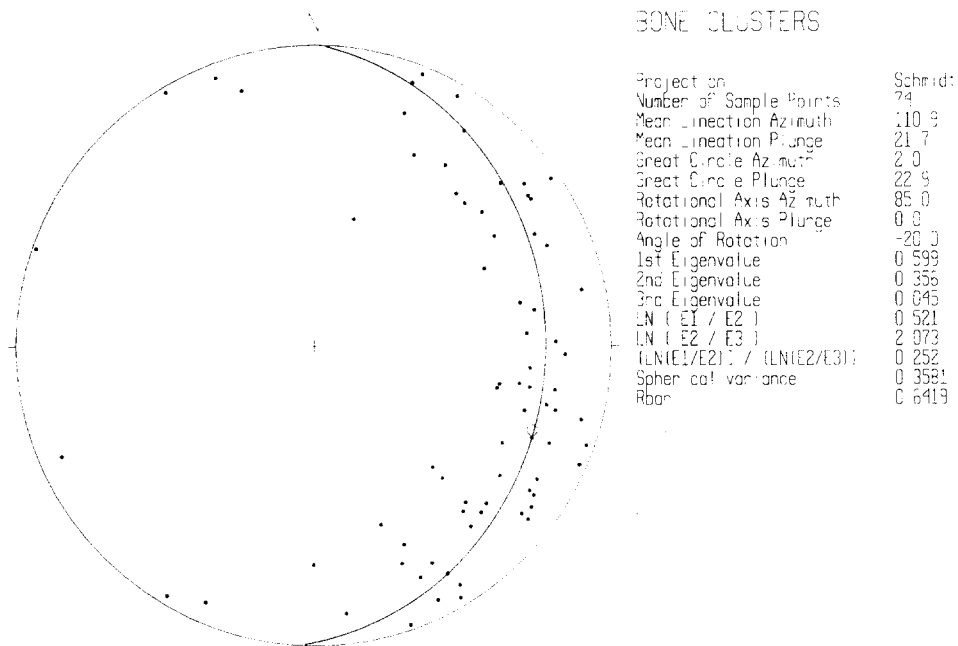
Fig. 6. Stereonet plot of rotated data on cormorant bones found in bone clusters in squares 2S4E, 3S4E and 4S3E illustrated in peaks of Fig. 5; only bones from the upper and lower shell are plotted. Note the strong directional orientation to the east for most bones in these clusters.
