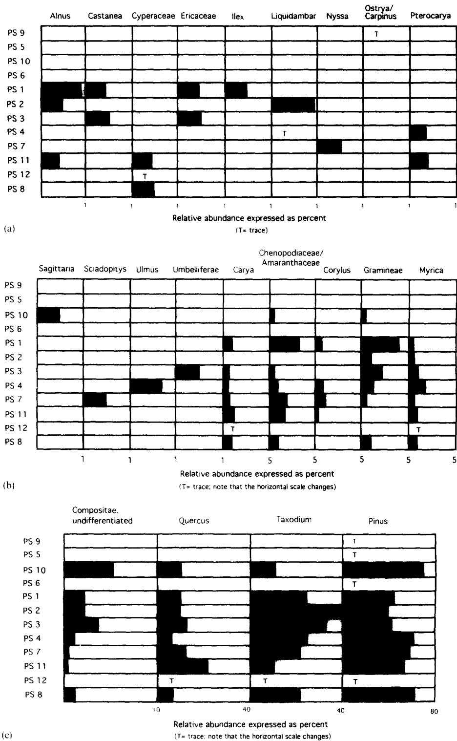
Fig. 9. Relative abundances of pollen in 12 samples (PS 1–12) from Richardson Road Shell Pit, Sarasota County, Florida. Samples are arranged on the vertical axis in stratigraphic order, top to bottom, with PS 9 from the highest unit (unit 2) and PS 8 from the lowest (unit 6/7; see Table 3). Trace means grains were seen in preliminary scans but were not observed during point counts.
