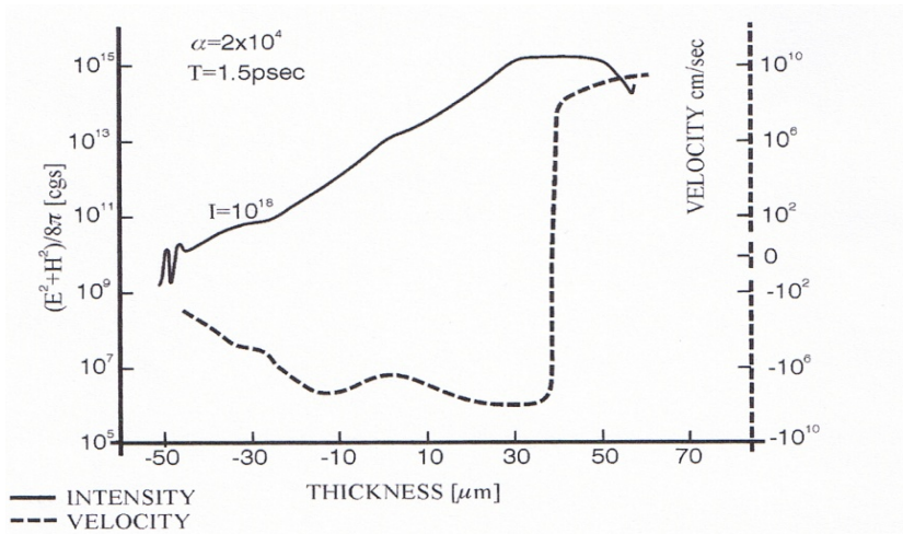
FIG. 1. 10^{18} \text{ W/cm}^2 neodymium glass laser is incident from the right hand side on an initially 100 \text{ eV} hot very low reflecting bi-Raleigh deuterium plasma profile at initial time t=0 , resulting at time t=1.5 \text{ ps} of interaction in a velocity distribution v(x) on the depth x and in an energy density of the laser field (\mathbf{E}^2 + \mathbf{H}^2)/8\pi . The dynamic development had accelerated the plasma block of about 20 vacuum wave length thickness of the skin layer moving against the laser and another block into the plasma showing ultrahigh >10^{20} \text{ cm/s}^2 dielectric enlarged acceleration [8].
