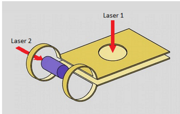
Fig 3. Reaction unit in the center of the reactor of Fig. 2 using “capacitor coil fields” producing a cylindrical magnetic field of kilotesla [22]. The cylindrical target with the HB11 fuel is co-axially located in a coil where during a ns the kilotesla magnetic field is produced by a kJ-ns laser pulse 1. A ps-30kJ laser pulse 2 initiates the non-thermal ignition of the fusion in the fuel.
