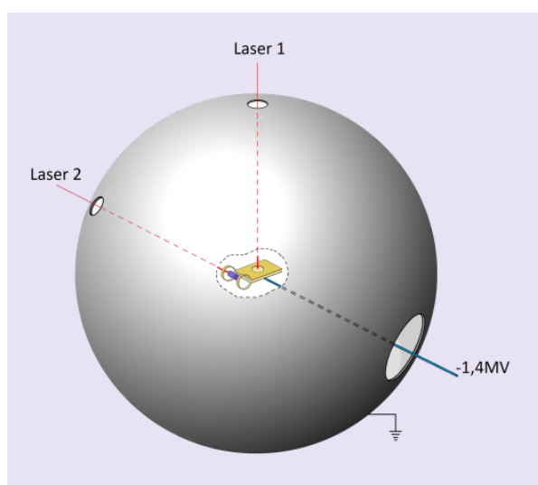
FIG. 2. Scheme of an economic electric power reactor for production of boron-fusion, with no problem of dangerous nuclear radiation with the estimated possibility of a power station producing low cost electricity [20]. The reaction unit in the center is described in Fig.3.
