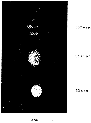
Fig. 1. Side-on framing camera picture of a plasma produced from an aluminum sphere of 80 \mu\text{m} radius at the time indicated after irradiation from the left hand side by a 30 \text{ ns} ruby laser pulse focused to 0.4 \text{ mm} diameter at the mentioned times after irradiation. The second frame shows a rapidly expanding half-moon-like plasma and a inner spherical part [5].
