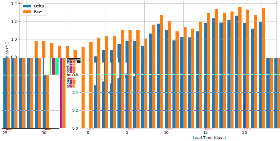
Figure S1. The mean absolute bias of temperature forecasts across lead times of 1-30 days.
