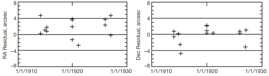
Figure B-39. Residuals of Pluto prediscovery observations.
