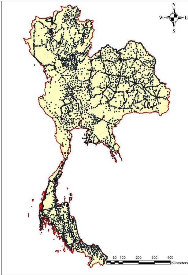
Figure 8 : Sub Earth's Gravity Stations
