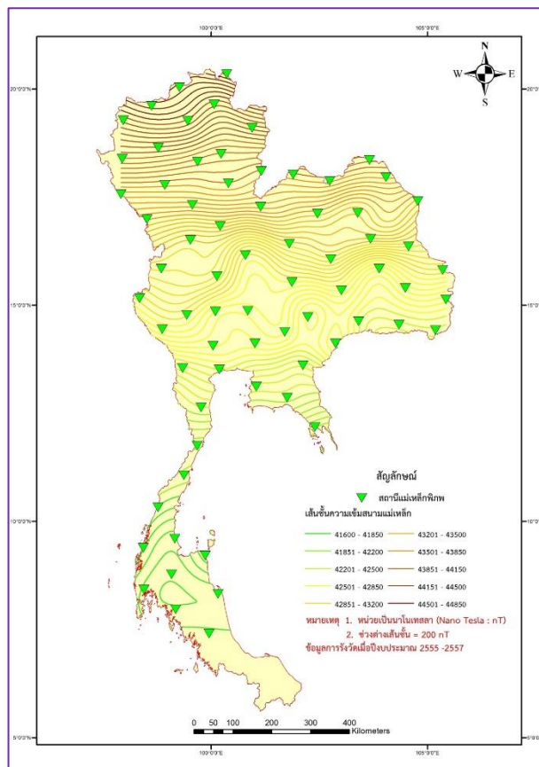
Figure 13 : Total Intensity Geomagnetic Chart
