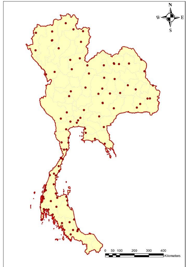
Figure 9 : Primary Earth's Gravity Stations
