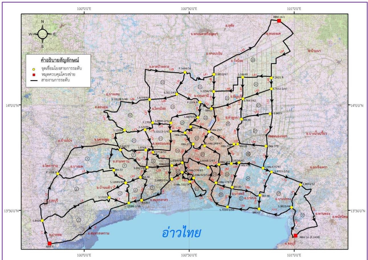
Figure 6 : First Order Leveling for Investigation of Land Subsidence in Bangkok
