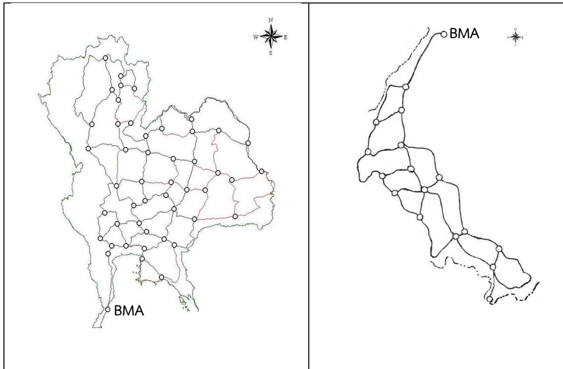
Figure 5 : First Order of Vertical Control Networks : Northern Part of Ko Lak Network (Left) and Southern Part of Ko Lak Network (Right)
