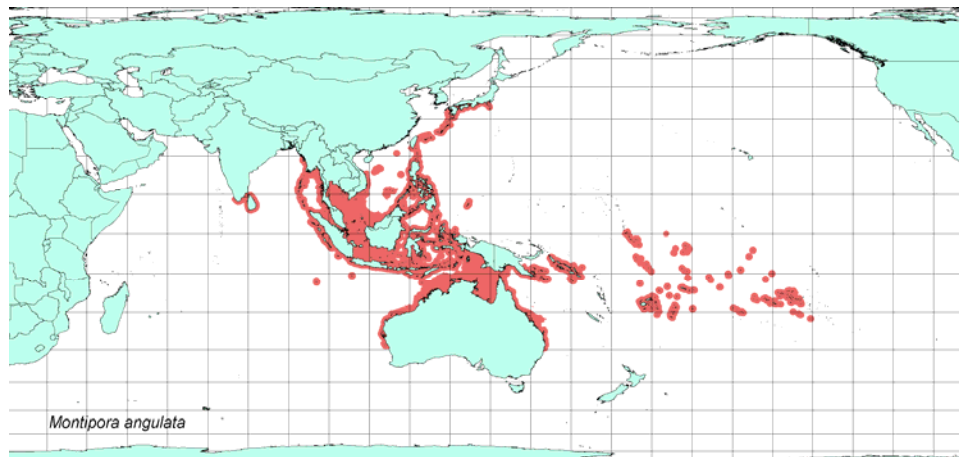
Figure 49. Range map for Montipora angulata .
