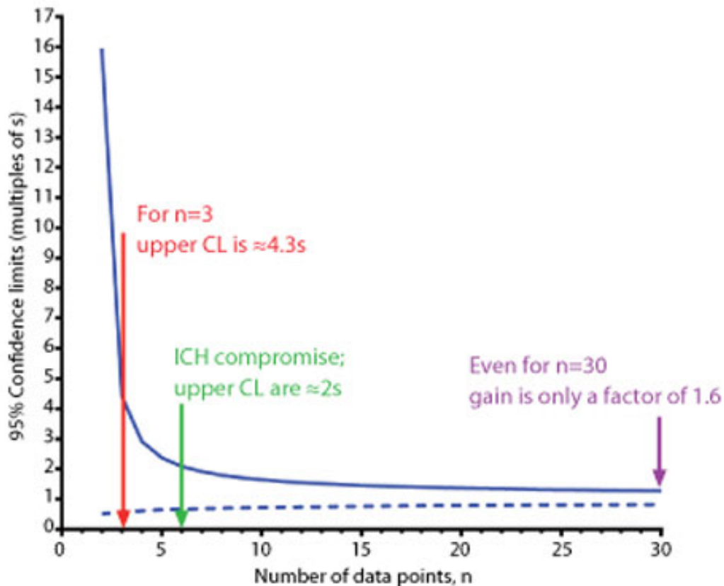
Figure 1: Effect of the number of samples (n) on the 95% confidence interval of the standard deviation expressed as multiples of itself (Burgess, 2014).
