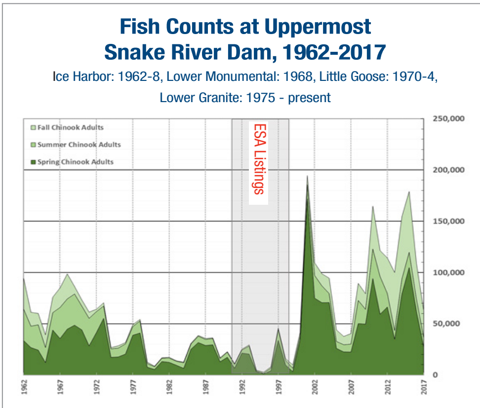
Figure 6. Combined returns of spring-summer, and fall Chinook salmon returning to the uppermost of the four lower Snake River dams, indicating the total number continuing on to spawning habitat in Idaho. From U.S. Army Corps of Engineers counts, accessed at www.cbr.washington.edu/dart .
