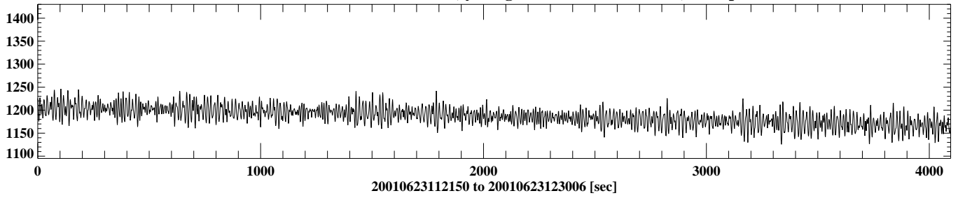
df00602200106231221 1 sec = dt, y range: 1104.7 - 1214.9 [cm], 4096 points
