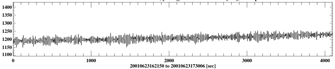
df00602200106231621 1 sec = dt, y range: 1147.9 - 1255.8 [cm], 4096 points
