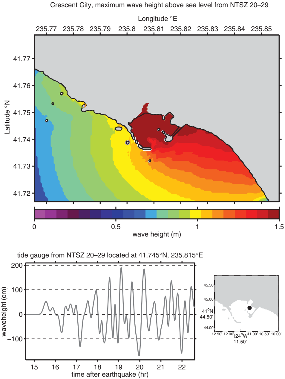
Figure 50: Maximum wave height plot and time series results for the forecast model using synthetic megatsunami Event NTSZ 20–29 for Crescent City, California.
