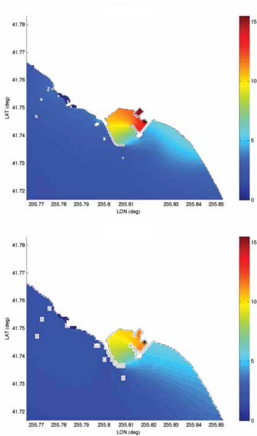
Figure 40: Maximum wave heights (cm) computed with forecast model grids. Asterisk indicates location of the tide gauge (reference model—upper, forecast model—lower) for the 2007 Peru event.
