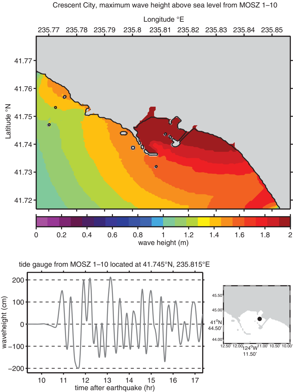
Figure 53: Maximum wave height plot and time series results for the forecast model using synthetic megatunami Event MOSZ 1–10 for Crescent City, California.
