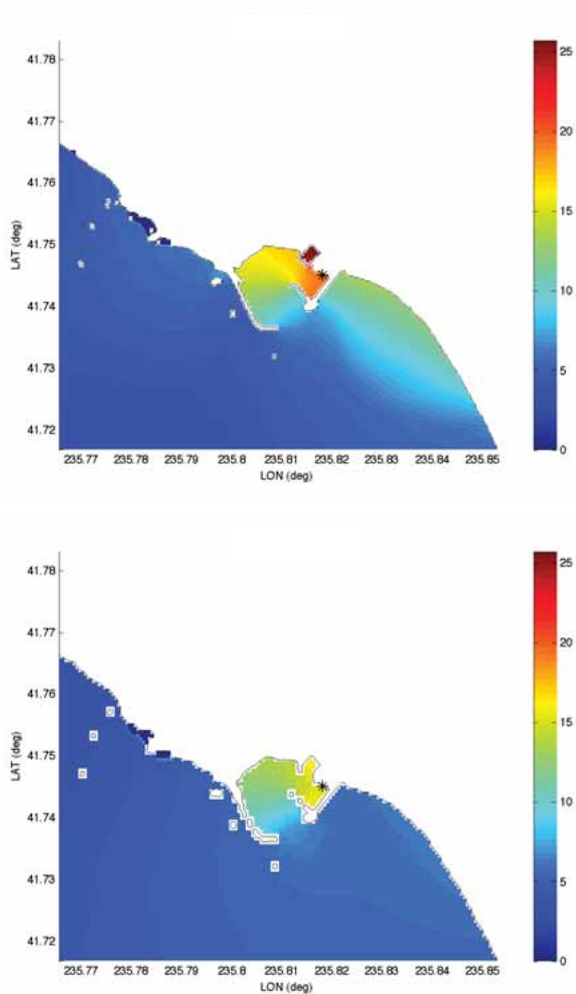
Figure 33: Maximum wave heights (cm) computed with forecast model grids. Asterisk indicates location of the tide gauge (reference model—upper, forecast model—lower) for the 1996 Andean event.
