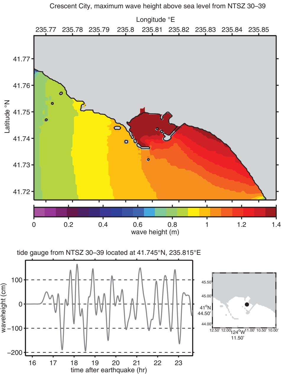
Figure 51: Maximum wave height plot and time series results for the forecast model using synthetic megatsunami Event NTSZ 30–39 for Crescent City, California.
