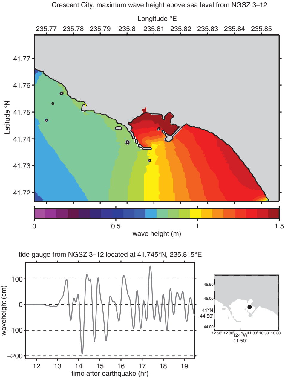
Figure 54: Maximum wave height plot and time series results for the forecast model using synthetic megatunami Event NGSZ 3–12 for Crescent City, California.
