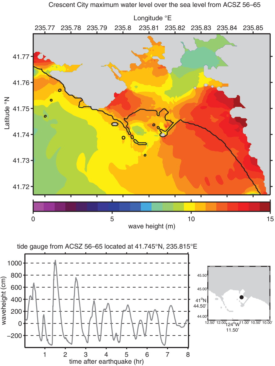
Figure 47: Maximum wave height plot and time series results for the forecast model using synthetic megatunami Event ACSZ 56–65 for Crescent City, California.
