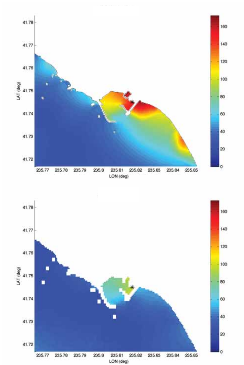
Figure 31: Maximum wave heights (cm) computed with forecast model grids. Asterisk indicates location of the tide gauge (reference model—upper, forecast model—lower) for the 1946 Unimak event.
