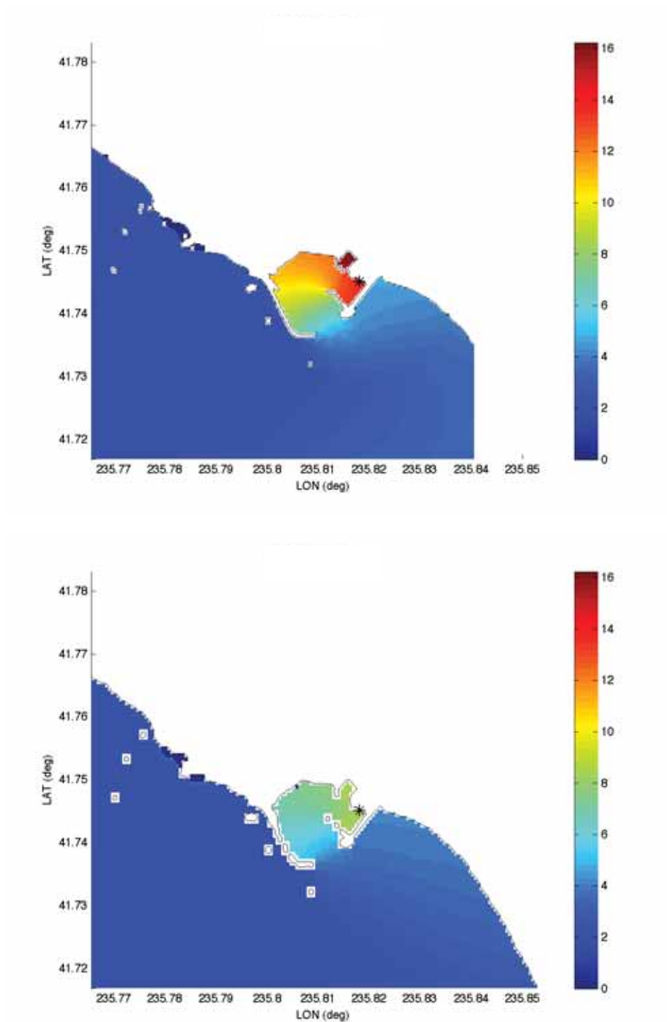
Figure 34: Maximum wave heights (cm) computed with forecast model grids. Asterisk indicates location of the tide gauge (reference model—upper, forecast model—lower) for the 2001 Peru event.
