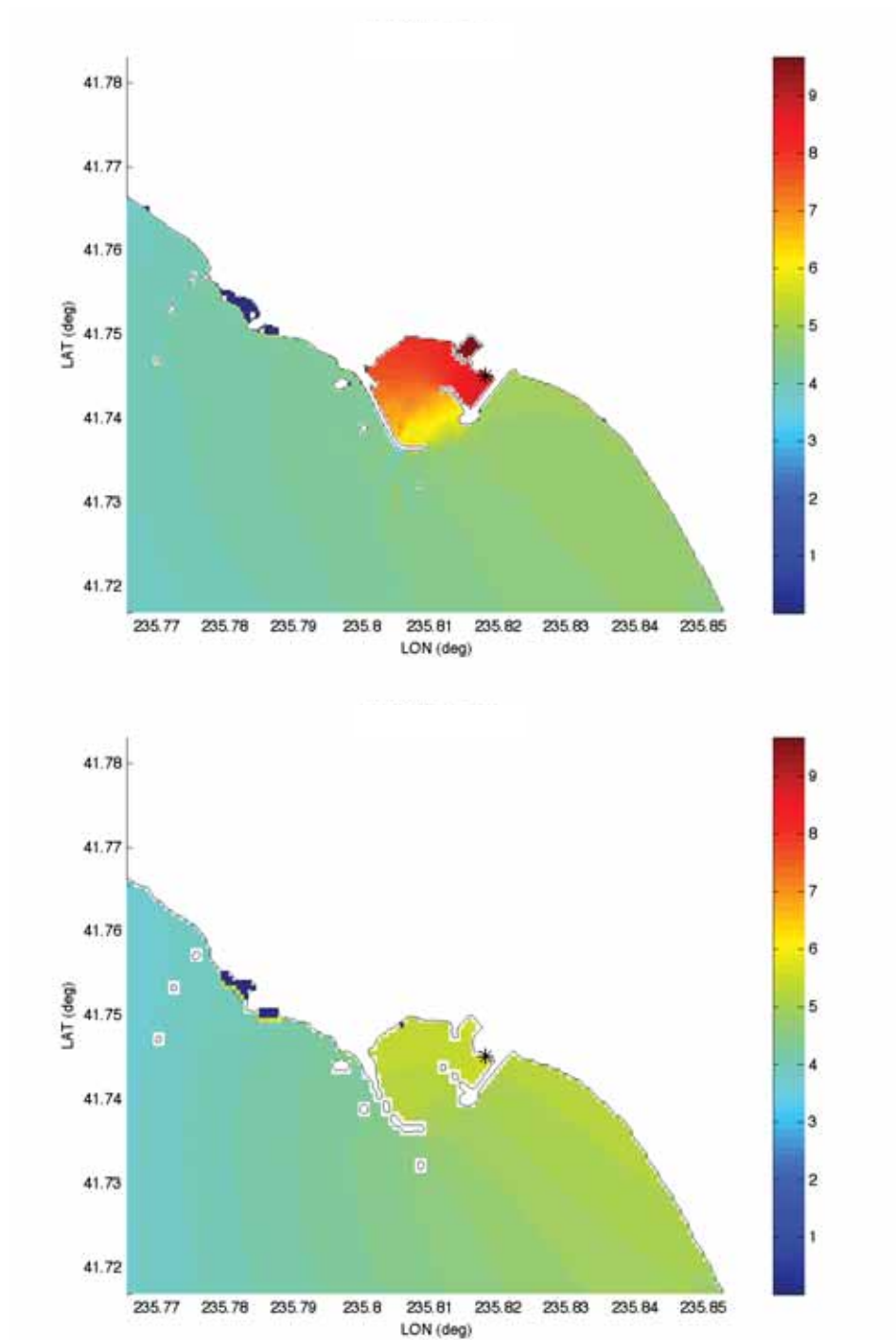
Figure 39: Maximum wave heights (cm) computed with forecast model grids. Asterisk indicates location of the tide gauge (reference model—upper, forecast model—lower) for the 2007 Solomon event.
