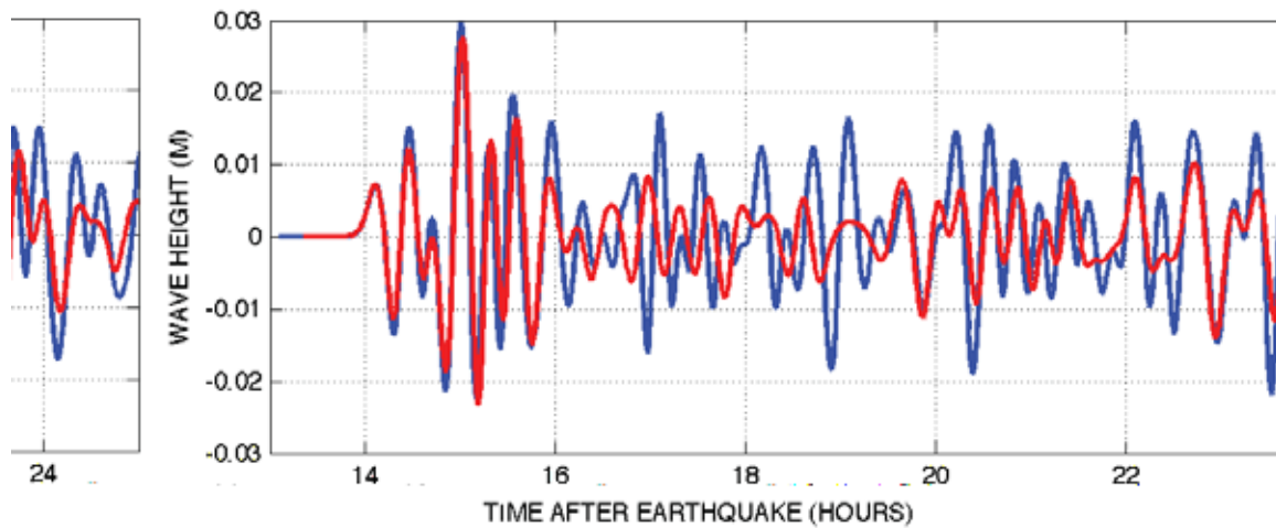
Figure 30: Time series comparison of reference vs. forecast model for the 2007 Chile event, blue—reference model, red—optimized forecast model.
