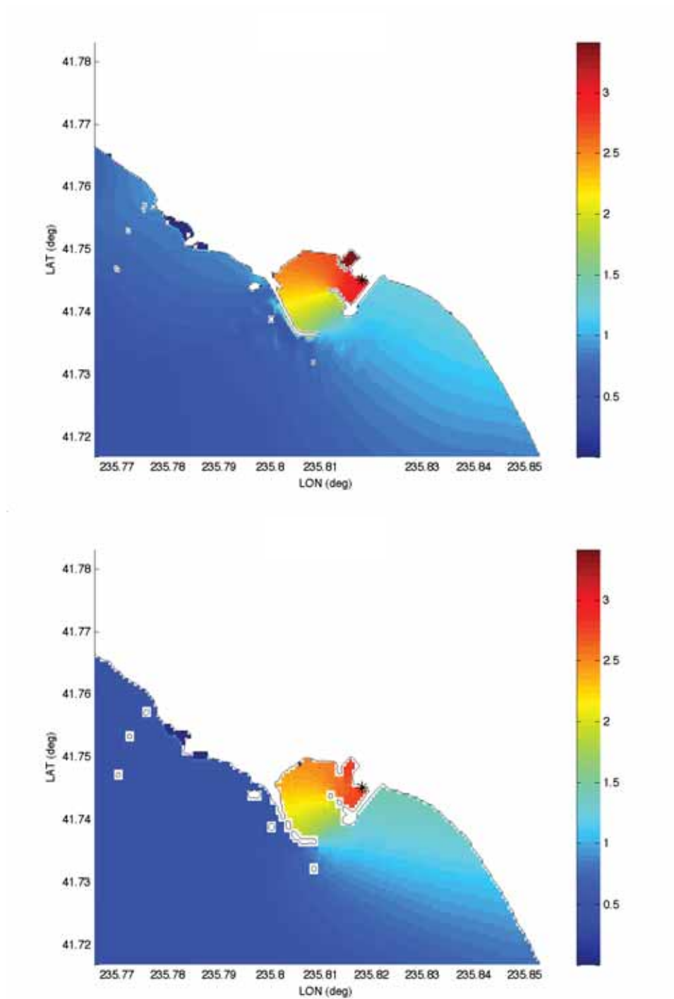
Figure 41: Maximum wave heights (cm) computed with forecast model grids. Asterisk indicates location of the tide gauge (reference model—upper, forecast model—lower) for the 2007 Chile event.
