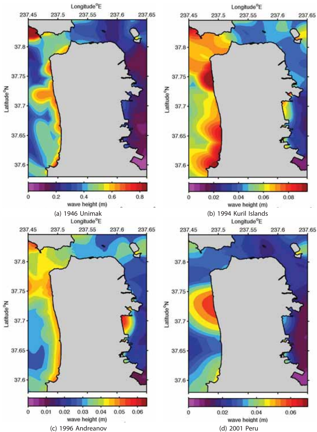
Figure 20: Maximum wave heights computed with reference model grids from (a) 1946 Unimak tsunami, (b) 1994 Kuril Islands tsunami, (c) 1996 Andeanov tsunami and (d) 2001 Peru tsunami.
