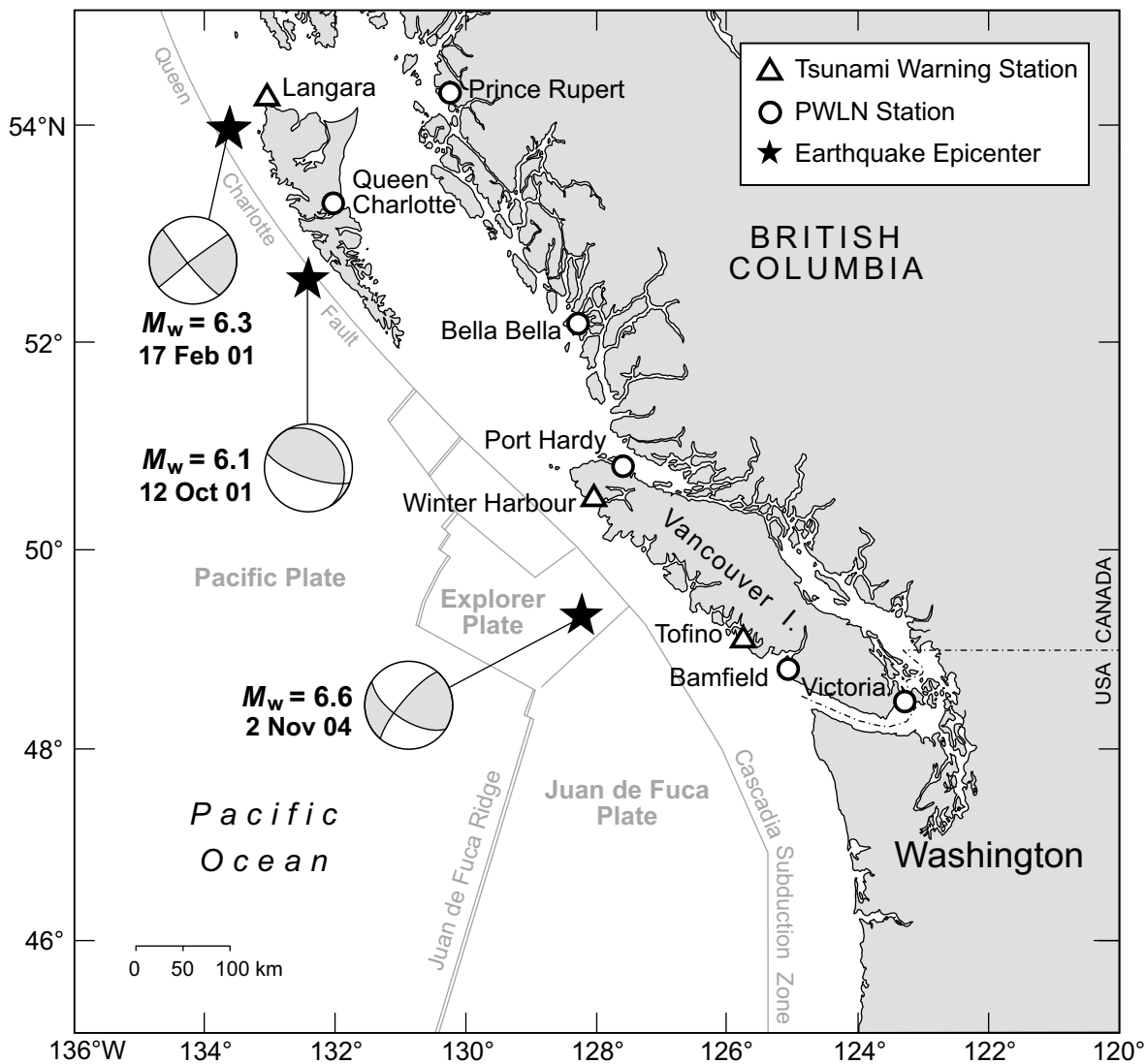
Fig. 1 Epicentres and fault mechanisms for the 12 October 2001 ( M_w = 6.1 ) and 2 November 2004 ( M_w = 6.6 ) tsunamigenic earthquakes. Also shown are the epicentre and fault mechanism for the 17 February 2001 ( M_w = 6.3 ) earthquake for which no tsunami was recorded. Circles denote locations of the Permanent Water Level Network (PWLN) tide gauges and triangles the Tsunami Warning tide gauge sites for the coast of British Columbia. Also shown are the positions of the main plates and faults.
