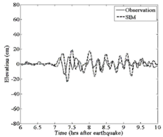
Figure 3. Comparison between observed water level and simulated SIM at Hilo for the 13 January 2007 Kuril event.
