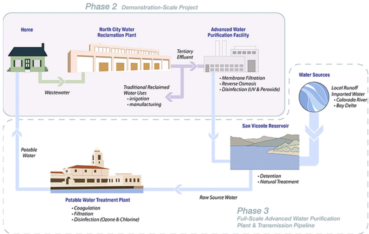
Figure 1 Water Purification Demonstration Process
