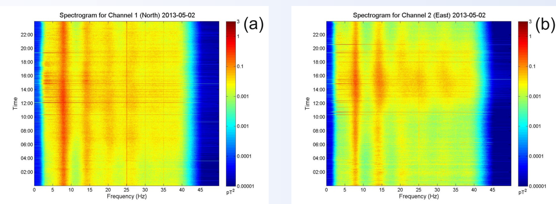
Figure 2: Butterworth bandpass-filtered (3-40Hz) data for 02-May-2013 for (a) Channel 1 (North) and (b) Channel 2 (East).
