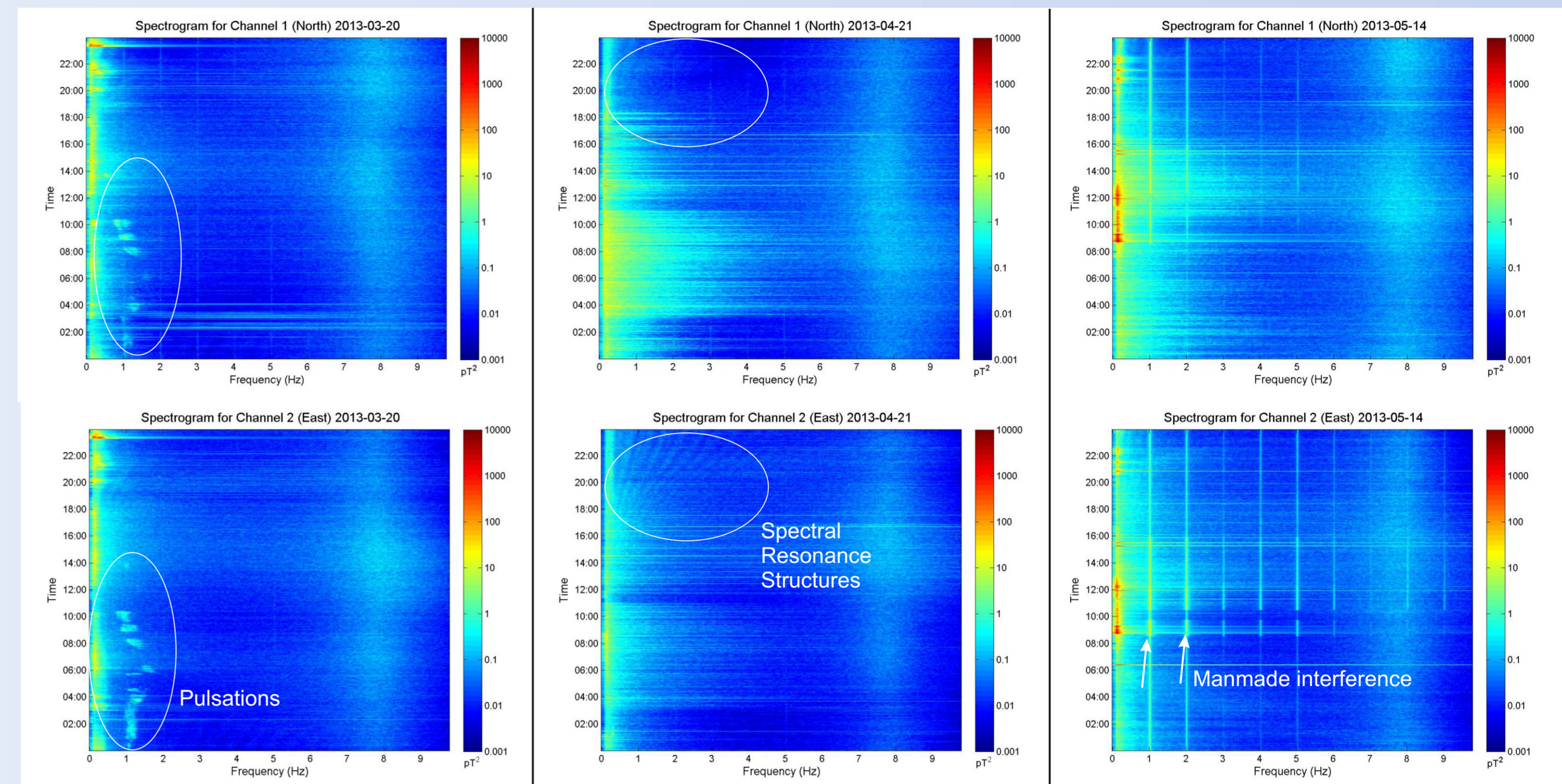
Figure 3: Butterworth bandpass-filtered (0.1-10Hz) data spectrograms showing magnetospheric pulsation activity (left panes) and fine Spectral Resonance Structures (middle panes) [2]. Also visible (right panes) is unexplained man-made interference presumably from electrical devices. Channel 2 is particularly sensitive to these effects. The first Schumann Resonance is visible around 8 Hz.
