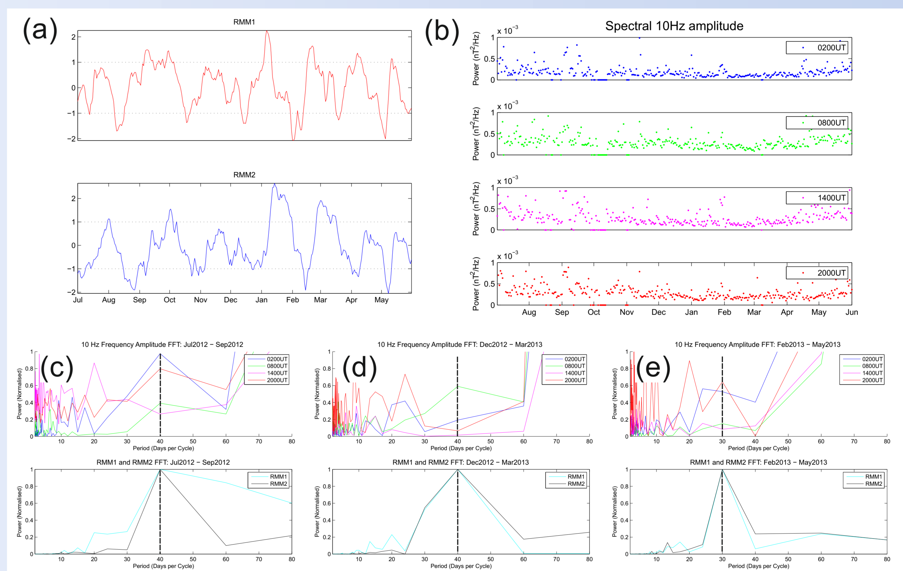
Figure 4: (a) Variation of the MJO Indices (RMM1 & 2) over 11 months. Values between dashed horizontal lines indicate weak MJO. (b) Variation of the amplitude of the 10 Hz spectral peak for each hour (02-0300UT, 08-0900UT, 14-1500UT and 20-2100UT) over 11 months. (c) FFT of the 10 Hz amplitudes for selected hours for 120 days between July and September 2012 and the RMM indices for the same period. A 40 day period exists in both the RMM and daytime 10 Hz amplitudes. (d) FFT of the 10 Hz amplitudes for each hour for 120 days between December 2012 and March 2013 and the RMM indices. Only the 0800UT curve shows a similar period. (e) FFT of the 10 Hz amplitudes for each hour for 120 days between February and May 2013 and the RMM indices for the same period. A 30 day period exists in both the RMM and 2000UT 10 Hz amplitude.
