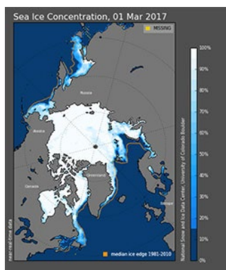
Figure 13a. Daily Sea Ice Concentration Image for the Northern Hemisphere.
