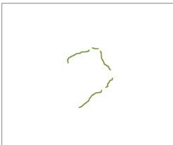
Figure 12a. Northern Hemisphere Median Shapefile for month of April, 1981 - 2010.
