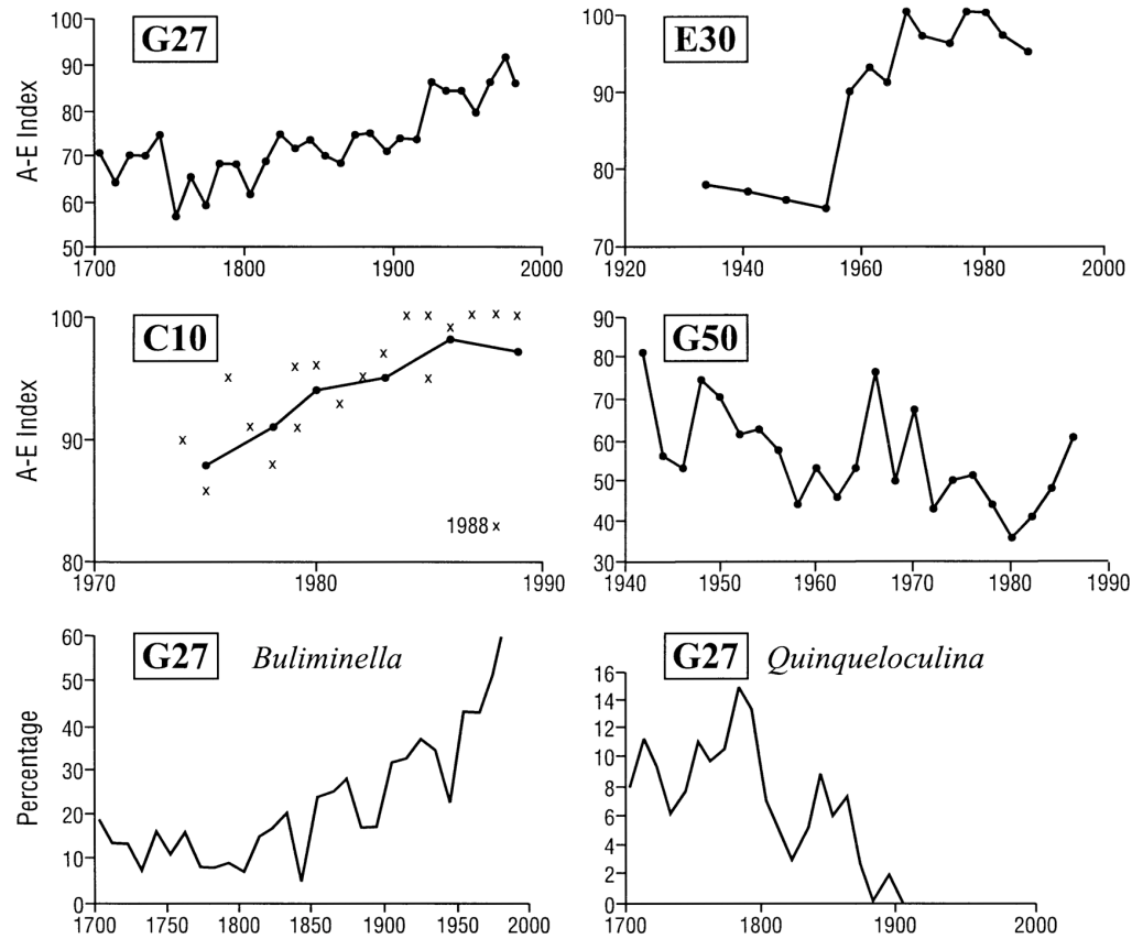
Figure 73. Changes in benthic foraminiferan species with stratigraphic depth in Pb-210 dated sediment cores from stations in the Mississippi River Bight. A line connecting 3-yr averages is superimposed on the data for C10. (Modified from Rabalais et al. 1996, Sen Gupta et al. 1996.)
