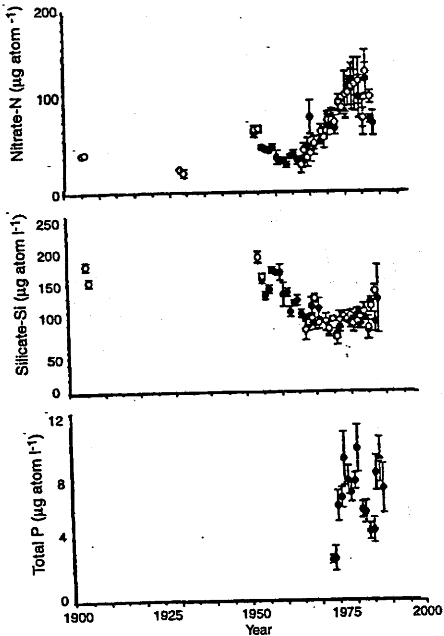
Figure 12. Nitrate, silicate and phosphorus concentrations measured at New Orleans (open circles) and St. Francisville (shaded circles). \pm 1 standard error bars are indicated for the annual average of monthly means. Figure adapted from Turner and Rabalais (1991)
