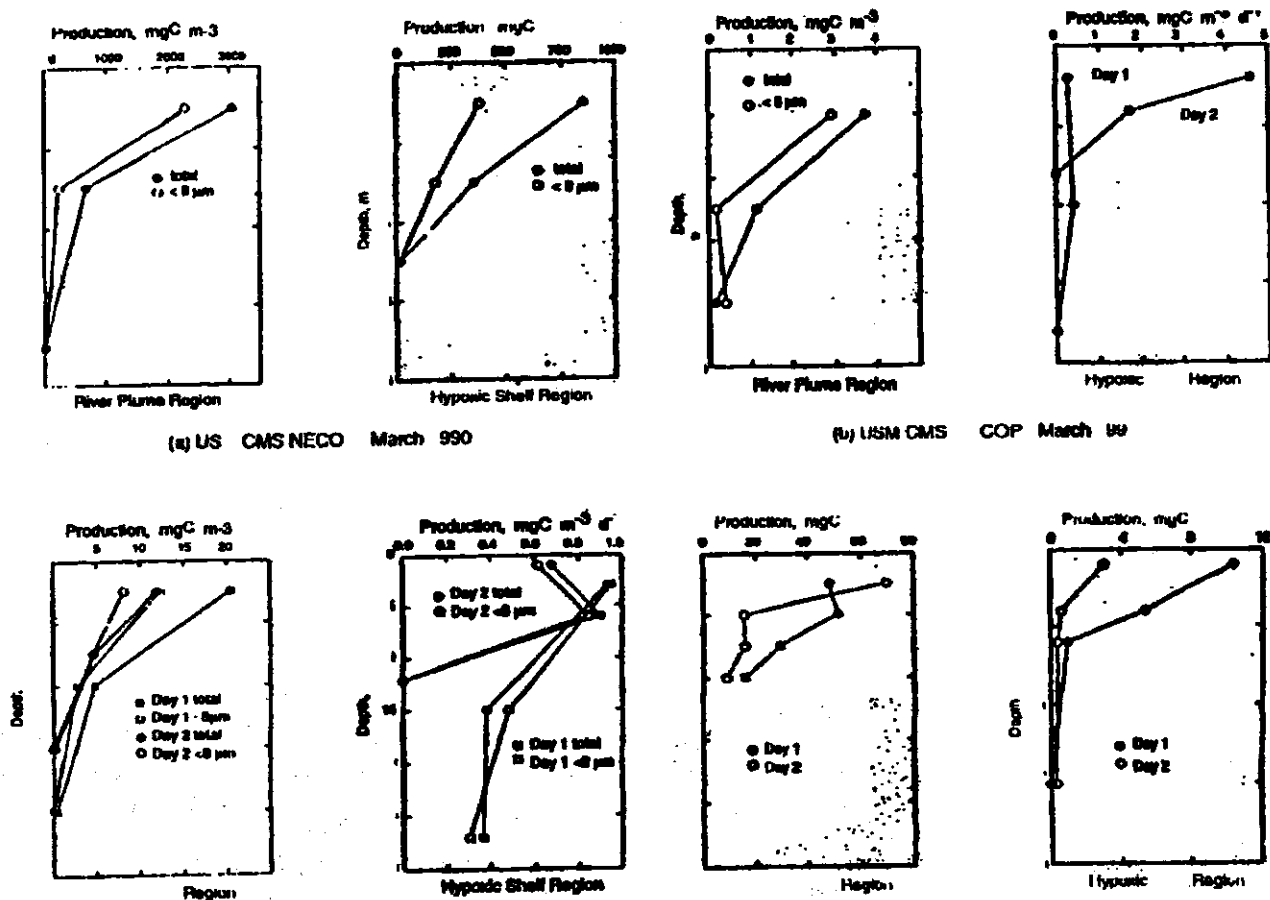
Figure 28. Size-fractionated phytoplankton production for phytoplankton < 8\mu\text{m} and phytoplankton > 8\mu\text{m} in size. Figure adapted from Redalje et al. (1994)
