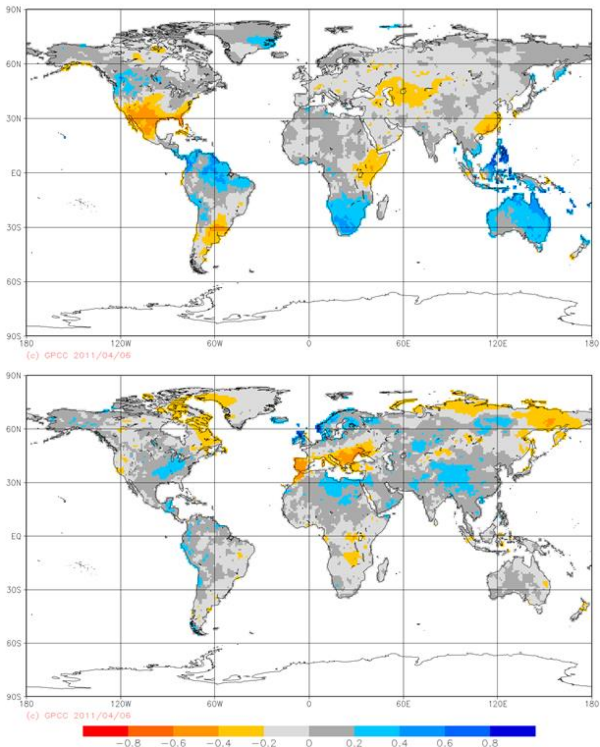
Figure 6: Correlation between monthly time series of gridded precipitation anomalies for the period 1901-March 2011 and (top) SOI and (bottom) NAO index (based on GPCCC Full Data Monthly V.5, 0.5° resolution, since Jan. 2010 Monitoring Product V.3)
