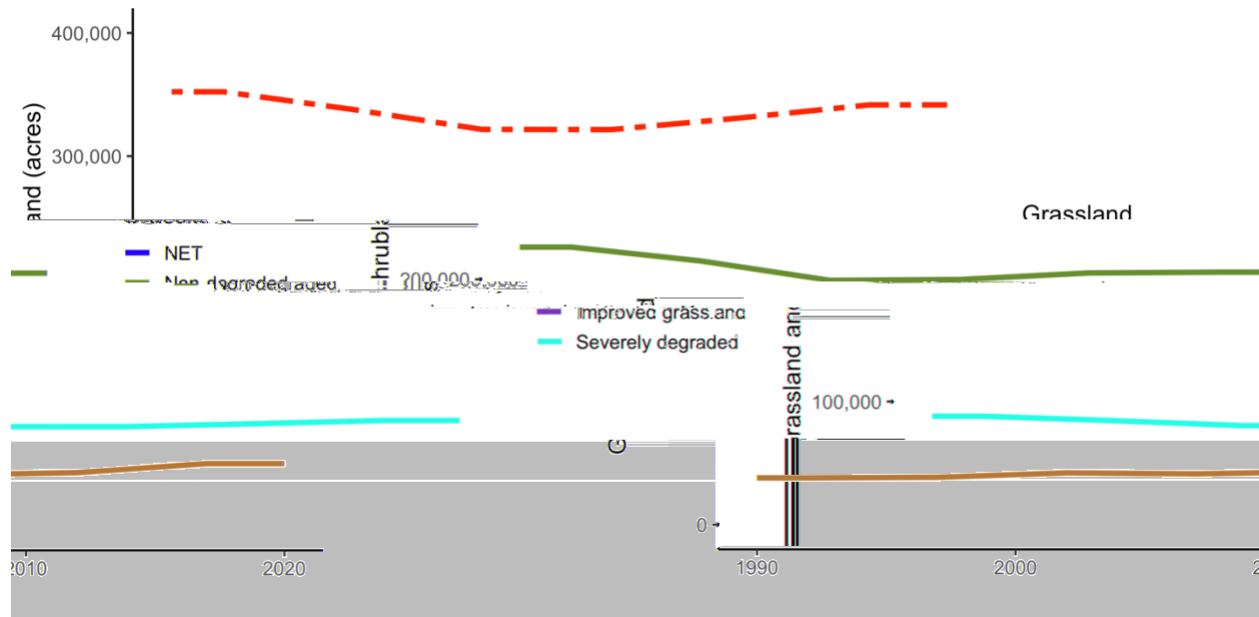
Figure 32: Estimated area of grasslands by condition 1990–2020
