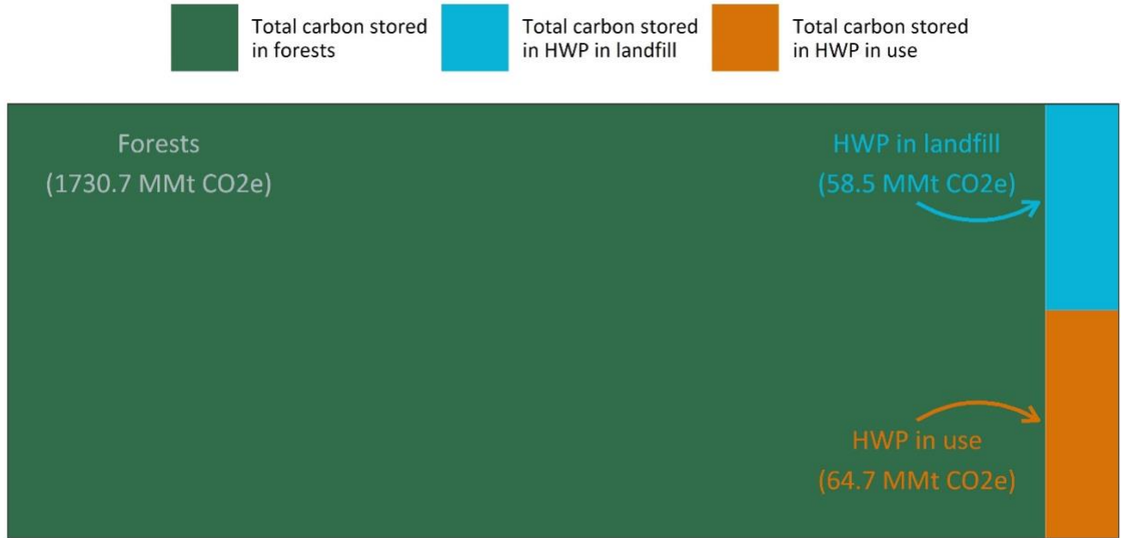
Figure 7: Estimated total carbon storage in Vermont’s forests and carbon stored in harvested wood products (HWP) both in use and in landfill
