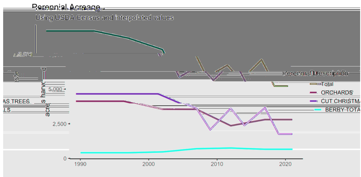
Figure 22: Area in specialty perennial crops (USDA NASS, 2021)
