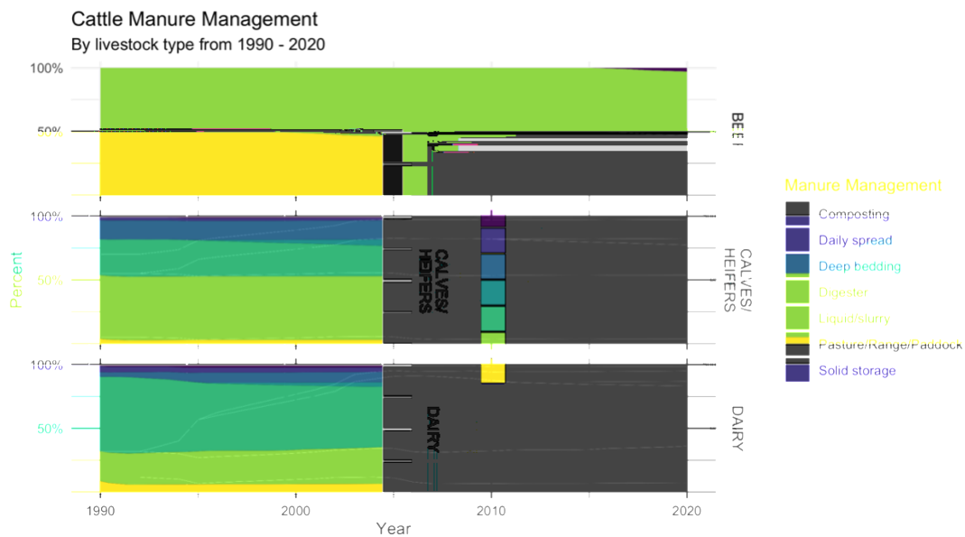
Figure 30: Changes in manure management by percent of total manure from cattle 1990–2020 based on expert knowledge
