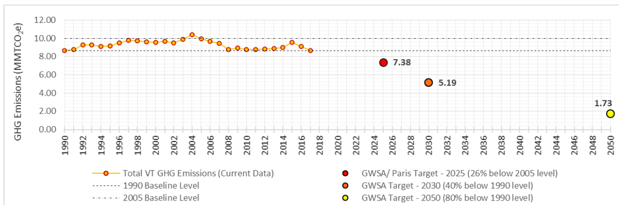
Figure 1: Vermont greenhouse gas emissions and mandated reduction targets as defined in the 2020 Global Warming Solutions Act 153 (GWSA) 10 V.S.A. § 578 (VT Agency of Natural Resources, 2021).
