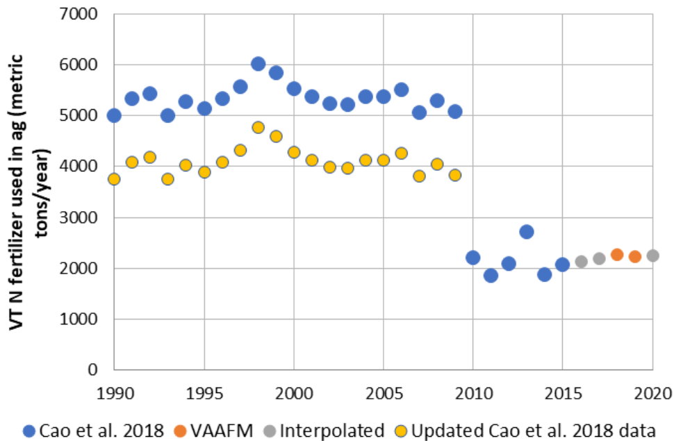
Figure 25: N-synthetic fertilizers used in Vermont agriculture 1990–2020, after Cao et al. 2018 and derived from VAAFM 2020, 2021
