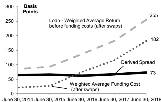
Figure 10: Derived Spread
