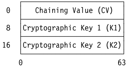
Figure 7-56. Parameter Block for KMAC-TDEA-128
