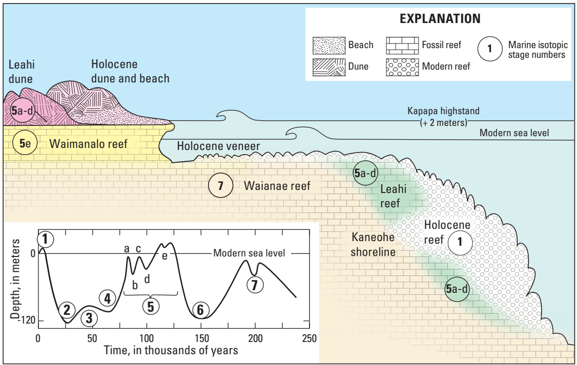
Figure 2. Principal stratigraphic components of the Oahu carbonate shelf. (Modified from Fletcher and others, 2008)
