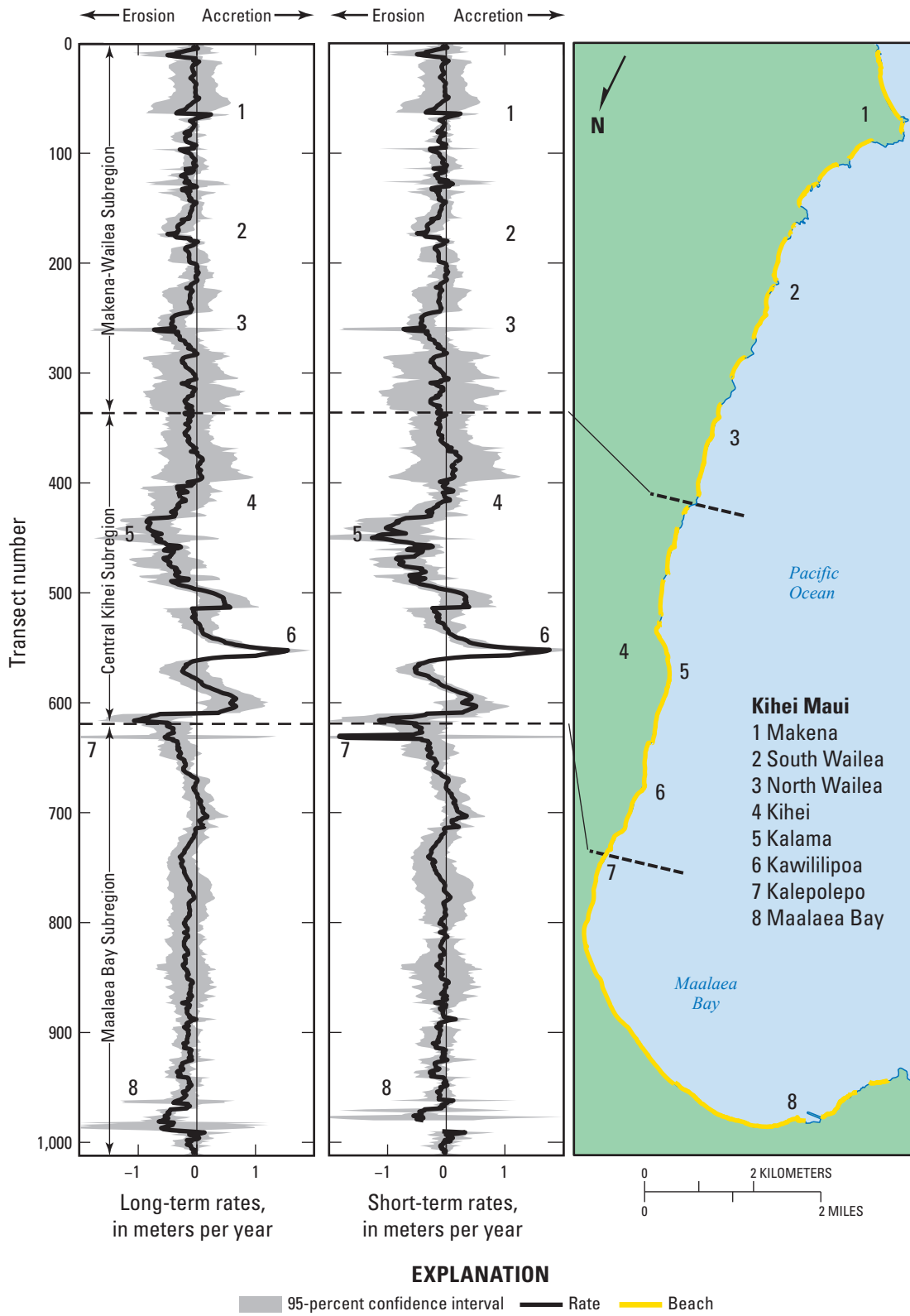
Figure 35. Long-term (all available years) and short-term (1940s to present) shoreline change rates, Kihei, Maui. (Location shown in figure 32)
