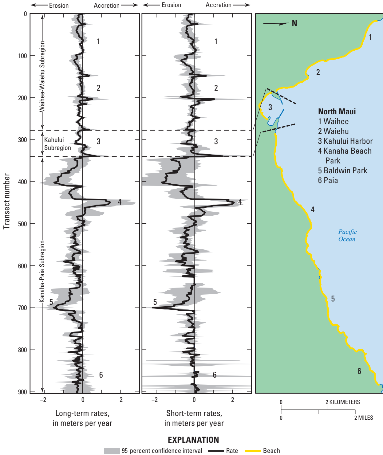
Figure 33. Long-term (all available years) and short-term (1940s to present) shoreline change rates, North Maui. (Location shown in figure 32)
