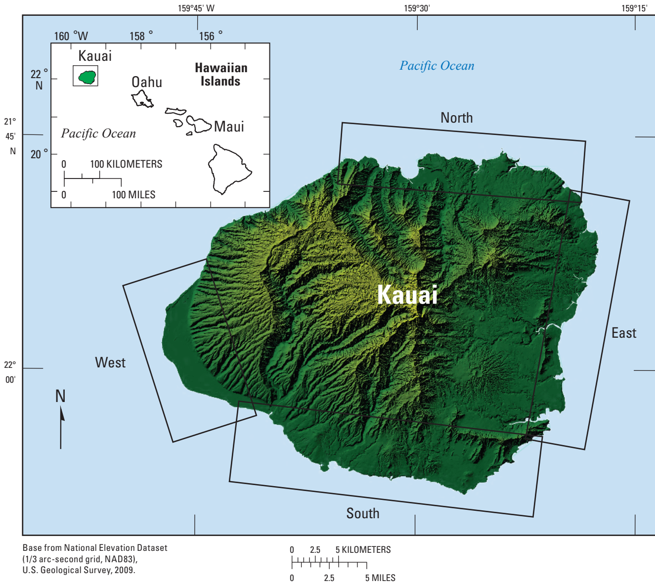
Figure 15. Four regions of Kauai: north, east, south, and west.
