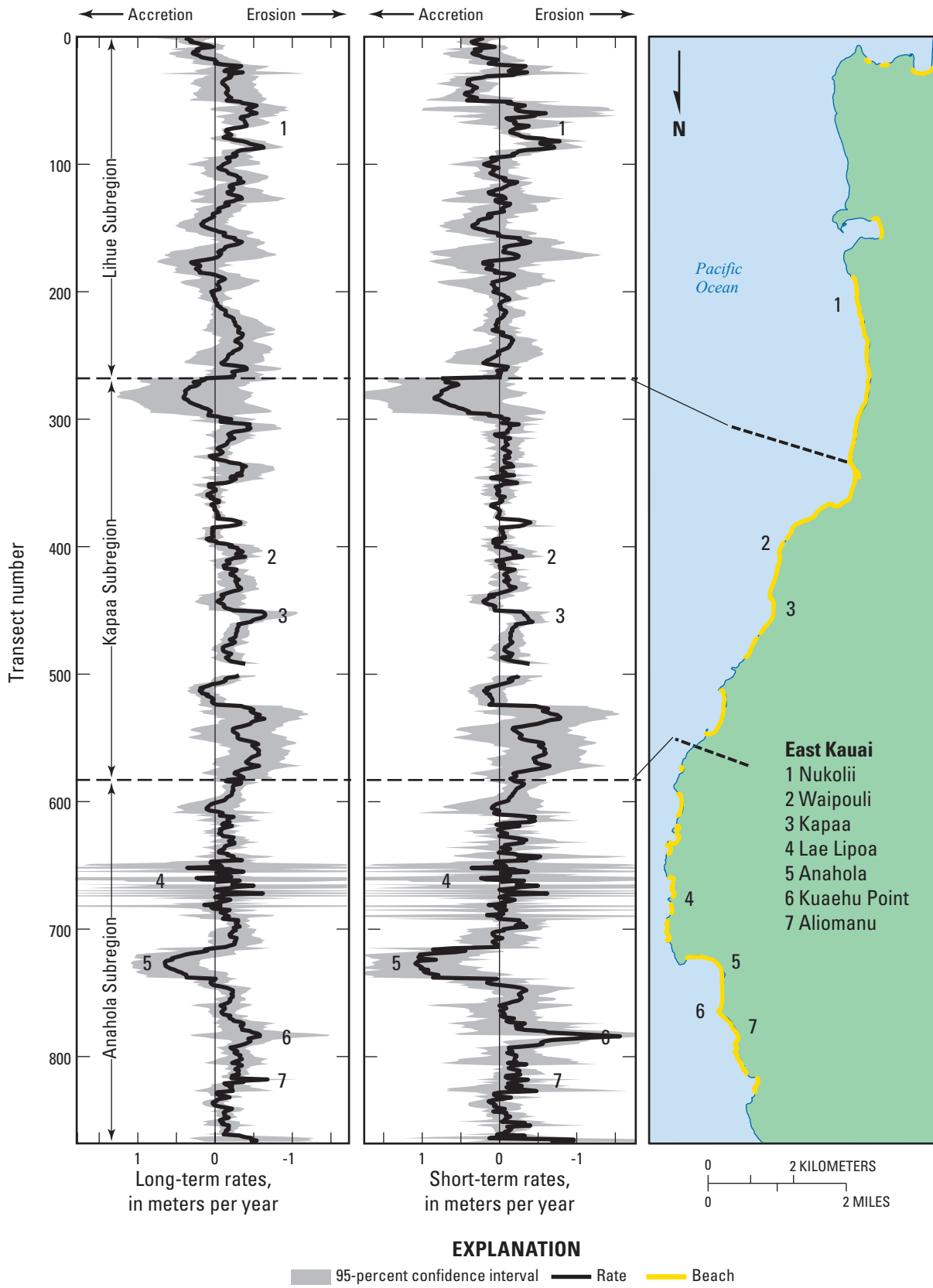
Figure 17. Long-term (all available years) and short-term (1940s to present) shoreline change rates, East Kauai. (Location shown in figure 15)
