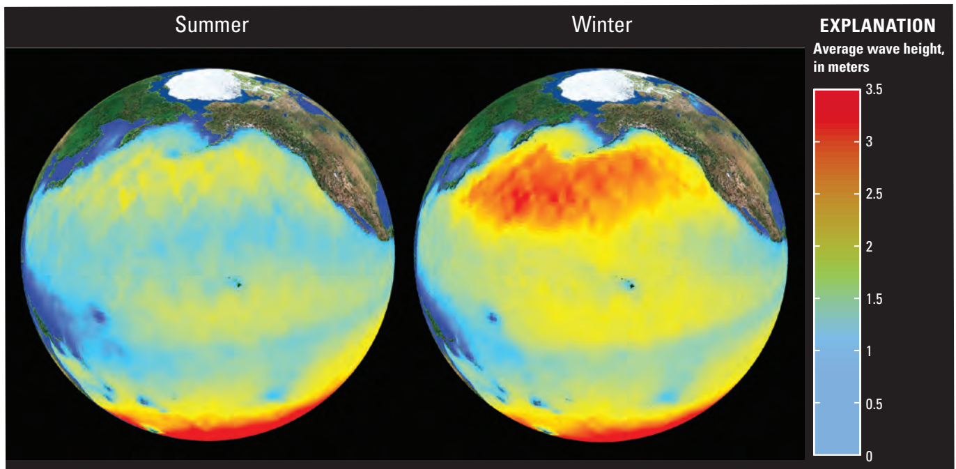
Figure 9. Satellite images (JASON-1) showing derived average wave height over the North Pacific in summer and winter. (National Oceanic and Atmospheric Administration, 2010)
