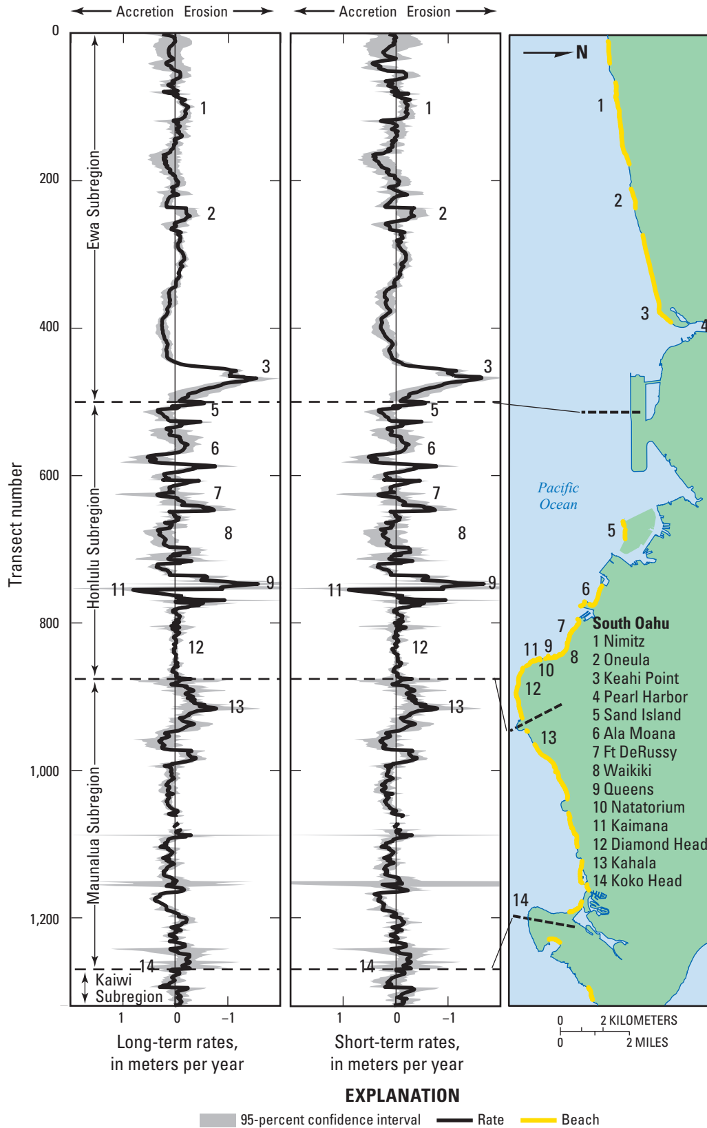
Figure 29. Long-term (all available years) and short-term (1940s to present) shoreline change rates, South Oahu. (Location shown in figure 22)
