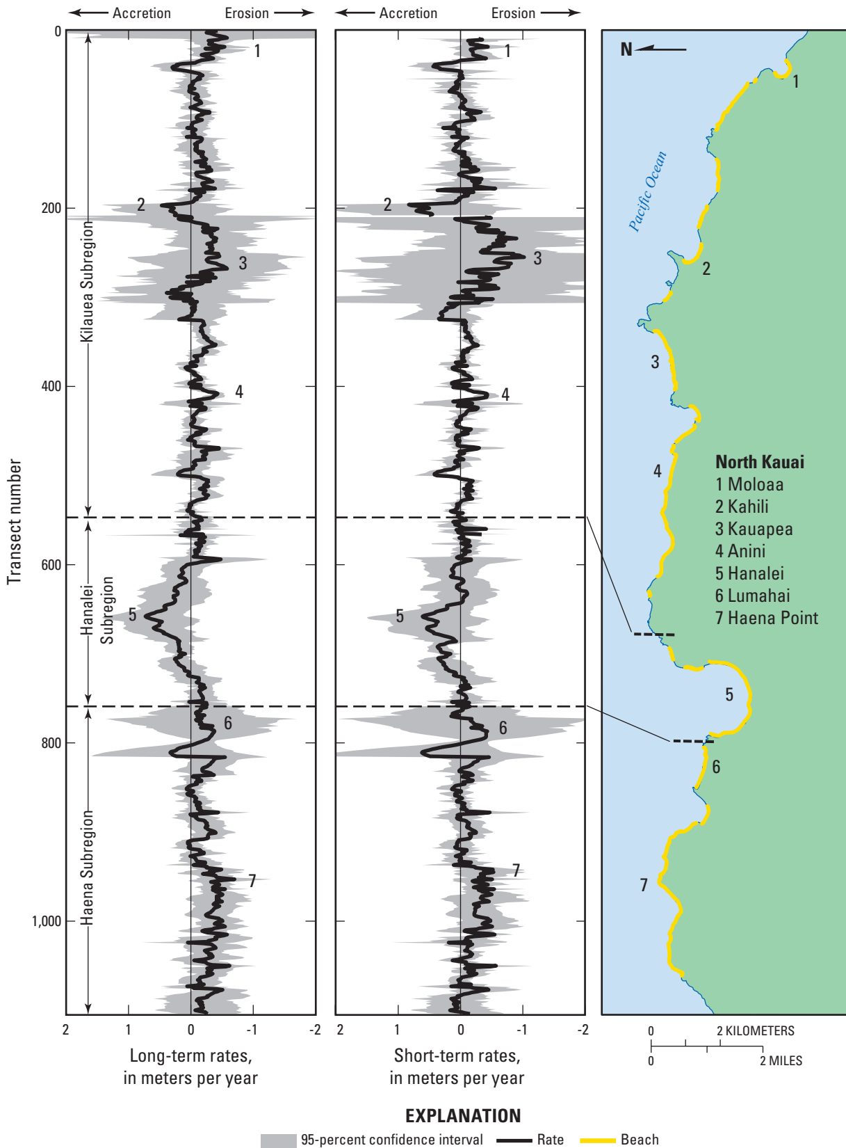
Figure 16. Long-term (all available years) and short-term (1940s to present) shoreline change rates, North Kauai. (Location shown in figure 15)
