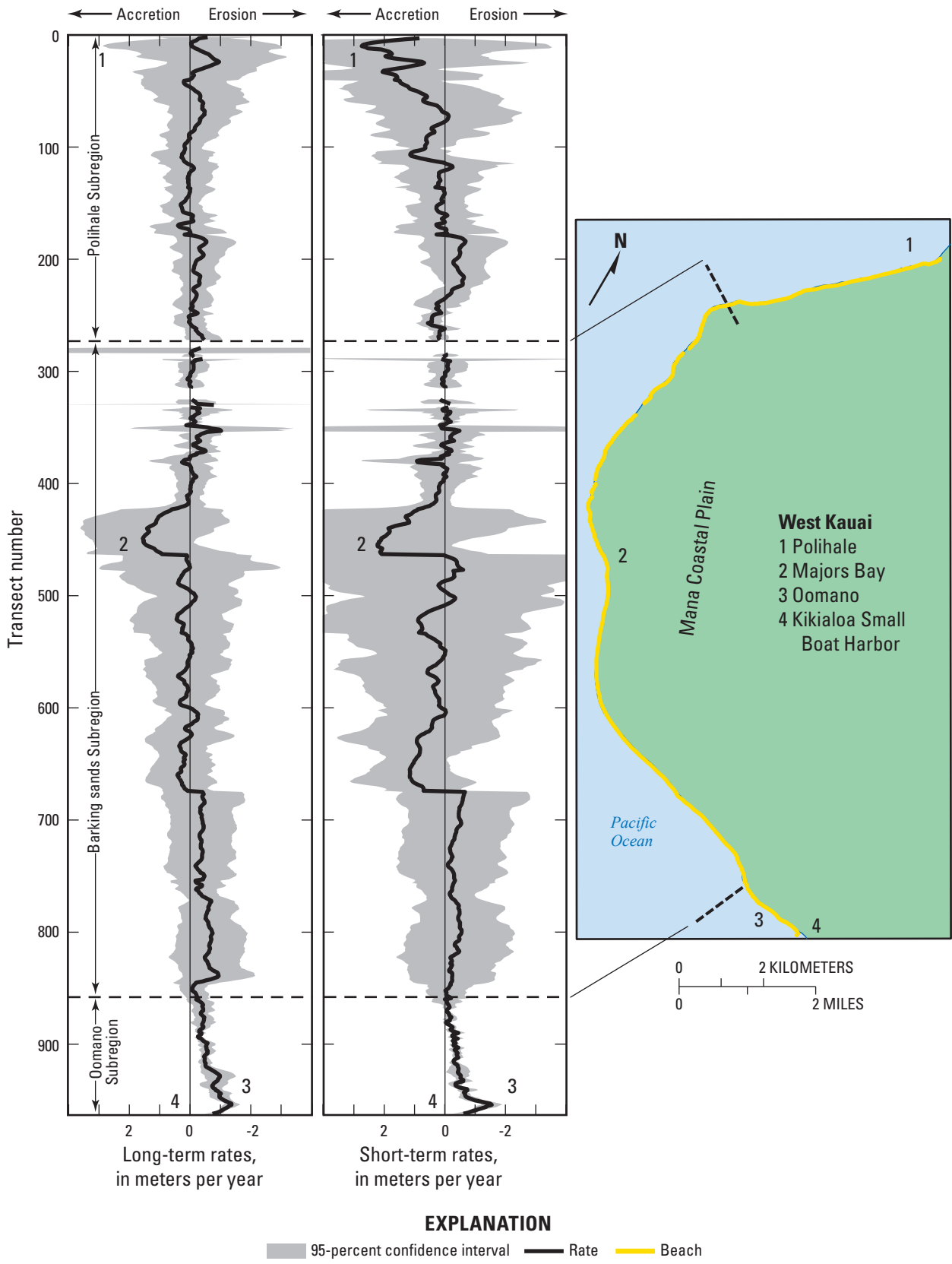
Figure 21. Long-term (all available years) and short-term (1940s to present) shoreline change rates, West Kauai. (Location shown in figure 15)
