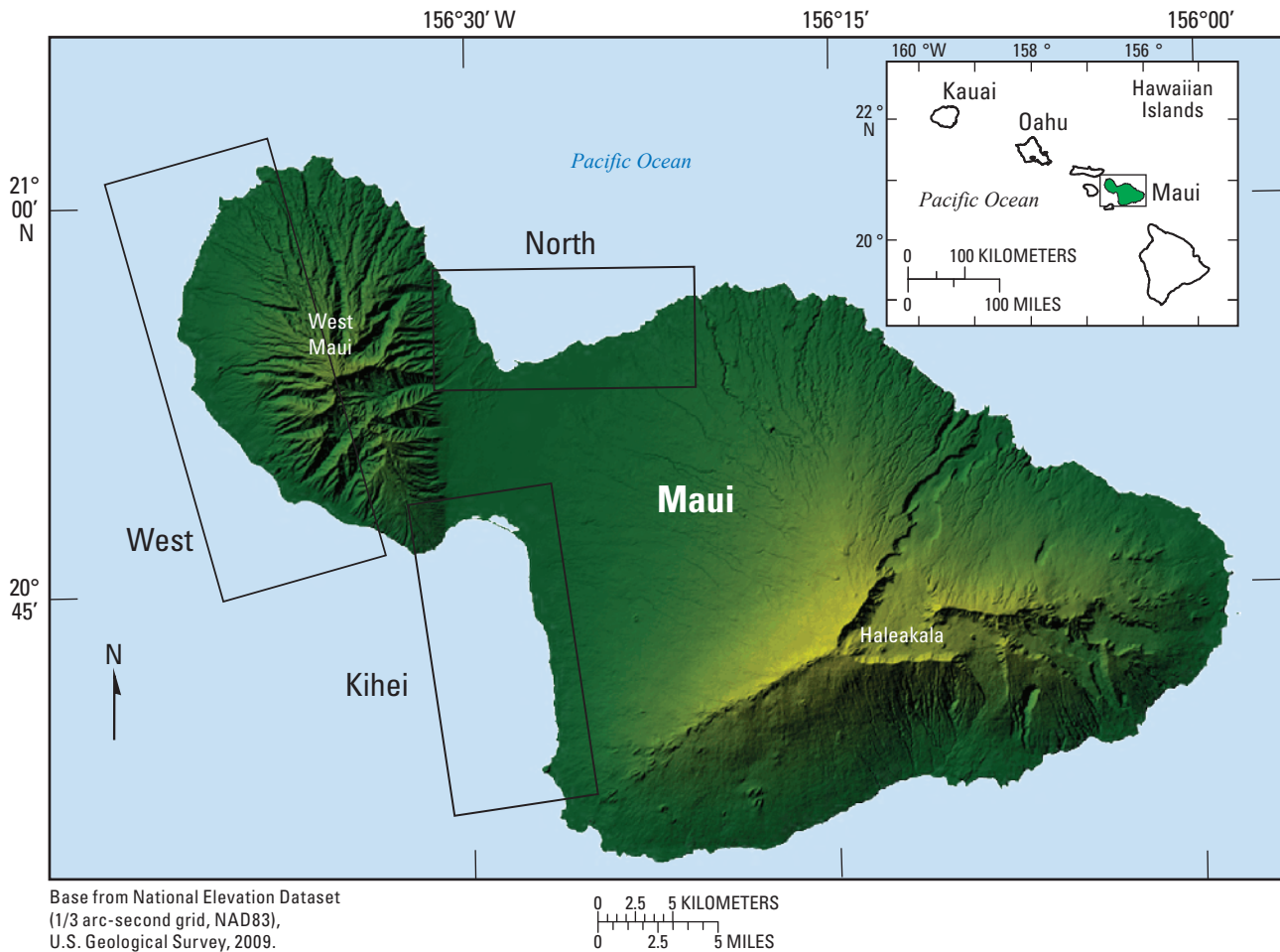
Figure 32. Three regions of Maui: north, Kihei, and west.
