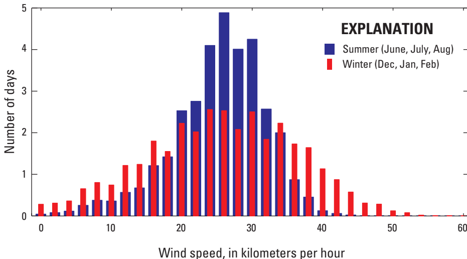
Figure 11. Number of days per season that trade winds occur with a particular speed (data from buoy 51001, 1981 to 2005). Note the persistence of typical trade winds at a speed of about 25 kilometers per hour (16 miles per hour) during summer months.
