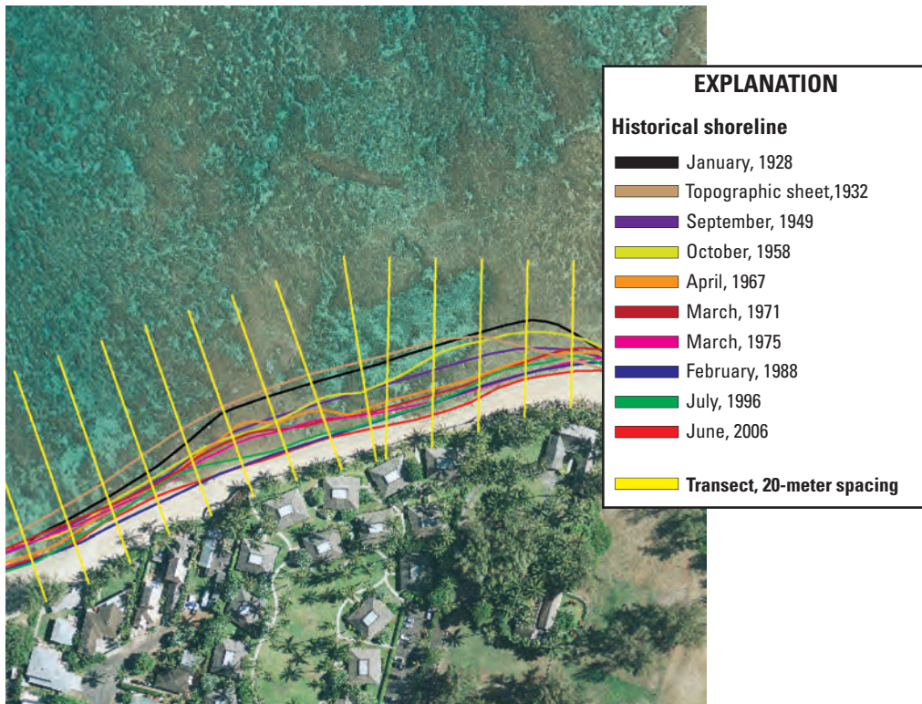
Figure 13. Historical shorelines and shore-perpendicular transects (20-meter spacing) displayed on a portion of a recent (2006) aerial photograph of Mokuleia Beach, North Oahu. (Location shown in figure 24) (Photograph by Hawaii Aviation, Inc.)
