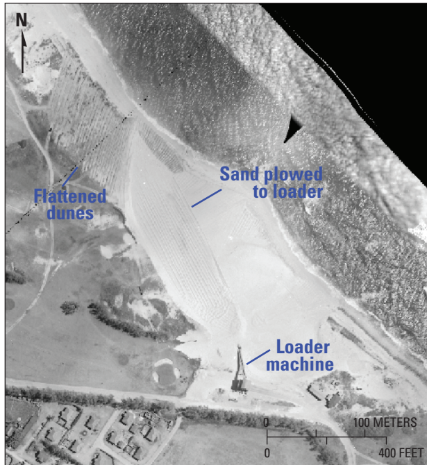
Figure 27. The south end of Kahuku Beach, northeast Oahu, 1949, showing evidence of sand mining. The dunes were flattened, plowed into the surf, and shoveled to the loading machine. The beach width decreased approximately 60 meters from 1949 to 1967. (Location shown in figure 26) (Photograph by R.M. Towill Corporation)
