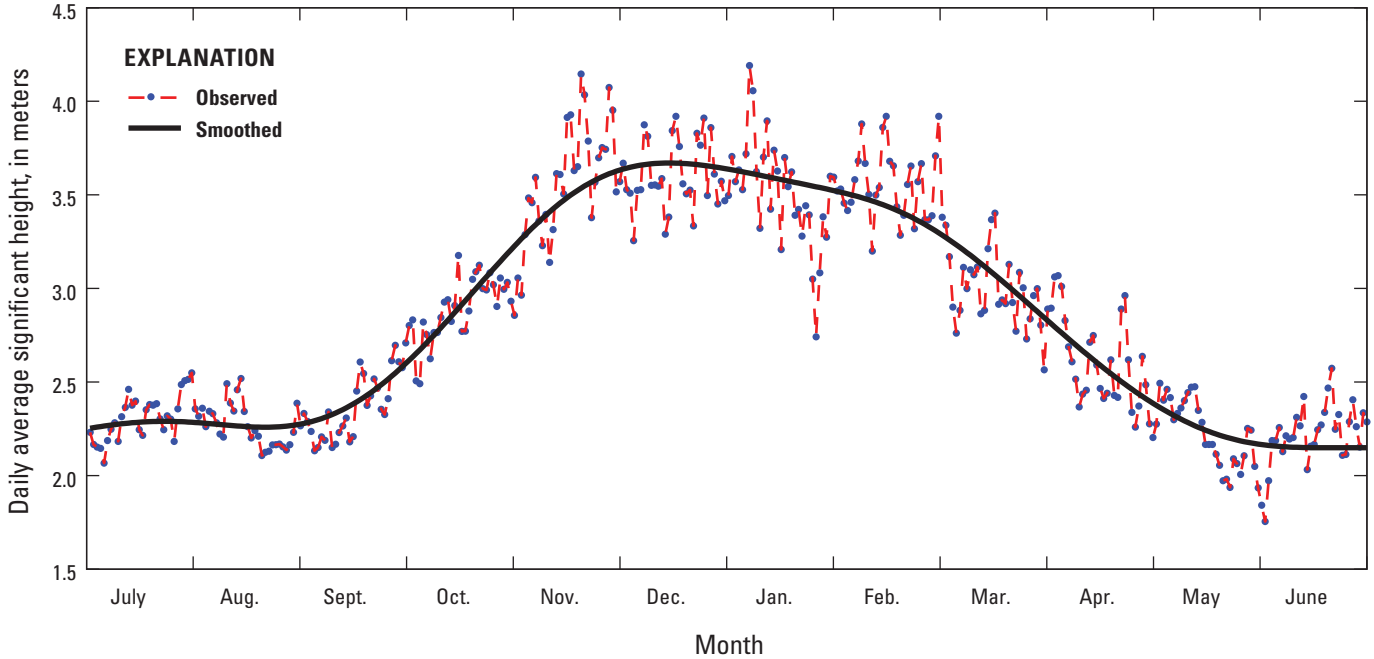
Figure 10. Daily average significant wave height from buoy 51001 (1981 to 2005, location shown in figure 8). This plot shows the seasonal variability of North Pacific Ocean swell, which begins to increase in October, reaches a peak in winter, decreases in March, and reaches a minimum in summer.
