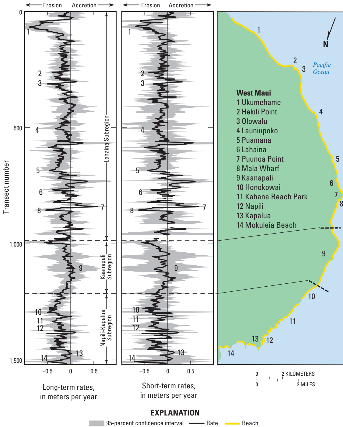
Figure 38. Long-term (all available years) and short-term (1940s to preset) shoreline change rates, West Maui. (Location shown in figure 32)
