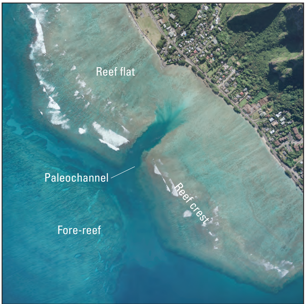
Figure 3. Carbonate sand beaches in Hawaii are the result of reef bioerosion and direct production of calcareous material by reef organisms. Reef morphology exerts strong control on shoreline sediment supply and dynamics. (Kaaawa, Oahu, location shown in figure 26) (Photograph by Hawaii Aviation, Inc., 2005)
