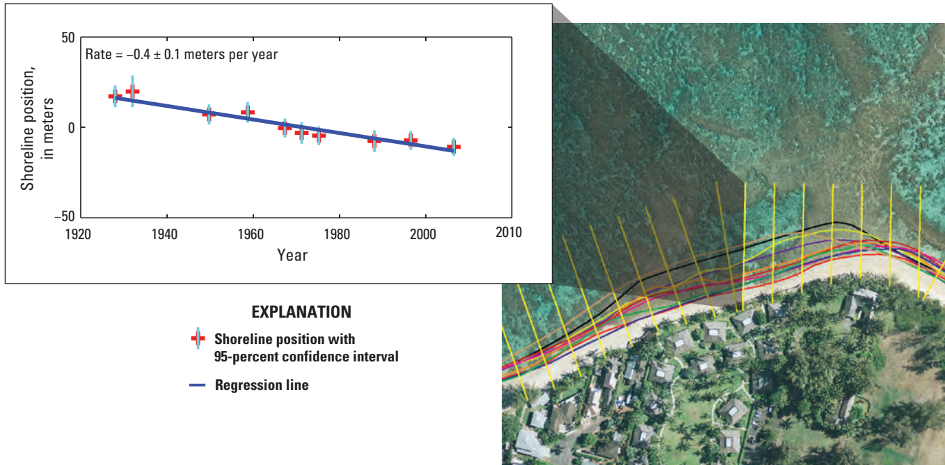
Figure 14. Calculation of shoreline change rate from a time series of shoreline positions using the single-transect method. The slope of the line is the annual shoreline change rate. (See figure 13 for explanation of photograph)
