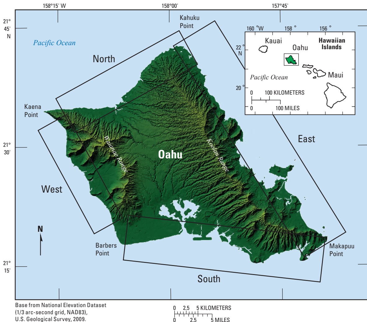
Figure 22. Four regions of Oahu: north, east, south, and west.
