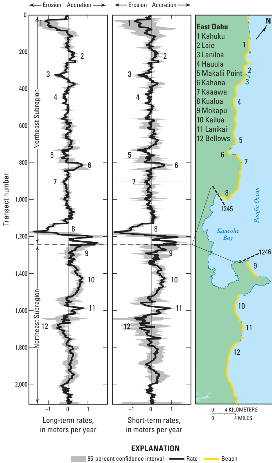
Figure 26. Long-term (all available years) and short-term (1940s to present) shoreline change rates, East Oahu. (Location shown in figure 22)
