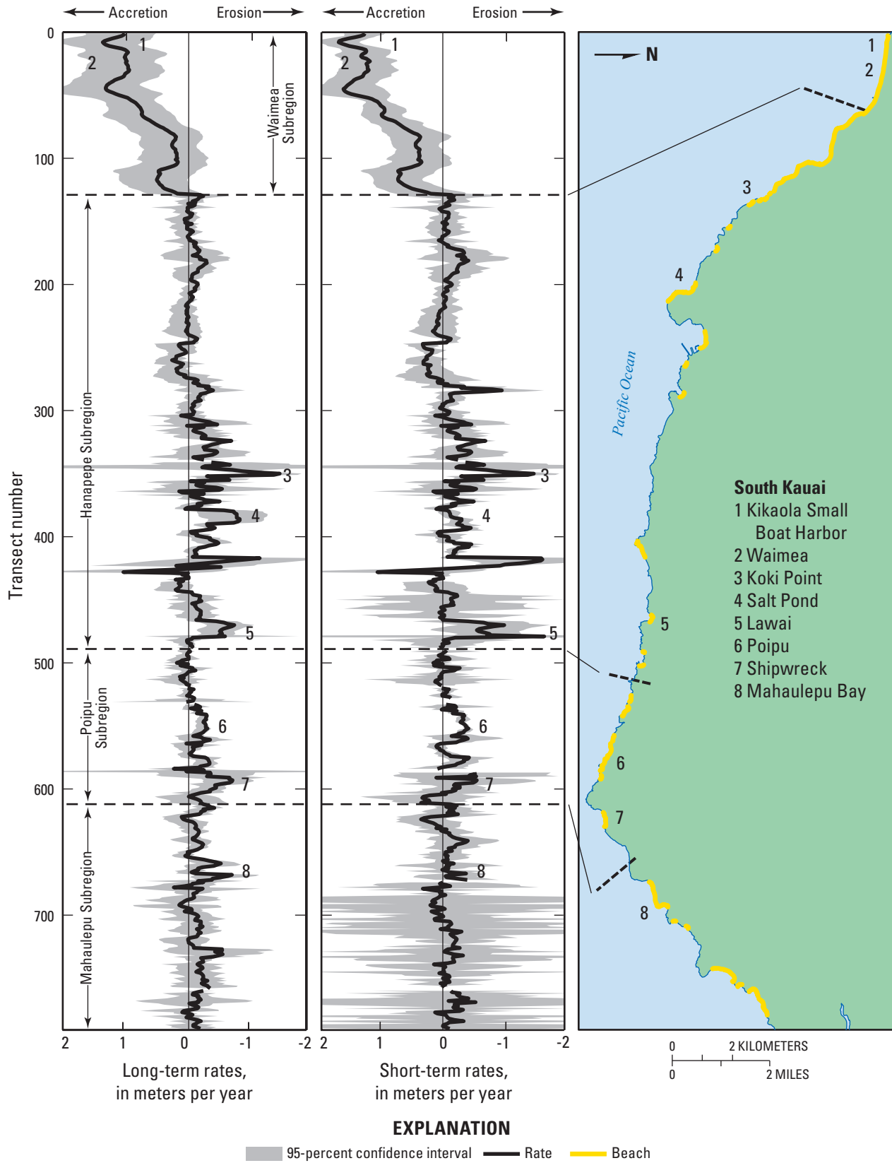
Figure 19. Long-term (all available years) and short-term (1940s to present) shoreline change rates, South Kauai. (Location shown in figure 15)
