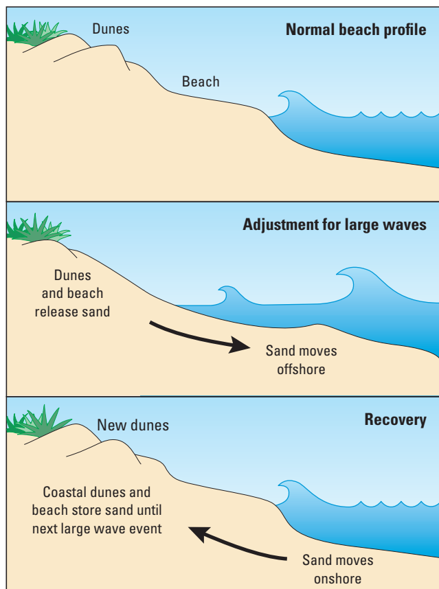
Figure 12. Seasonal beach-profile adjustments induced by seasonal swell variations and resulting cross-shore sediment transport.
