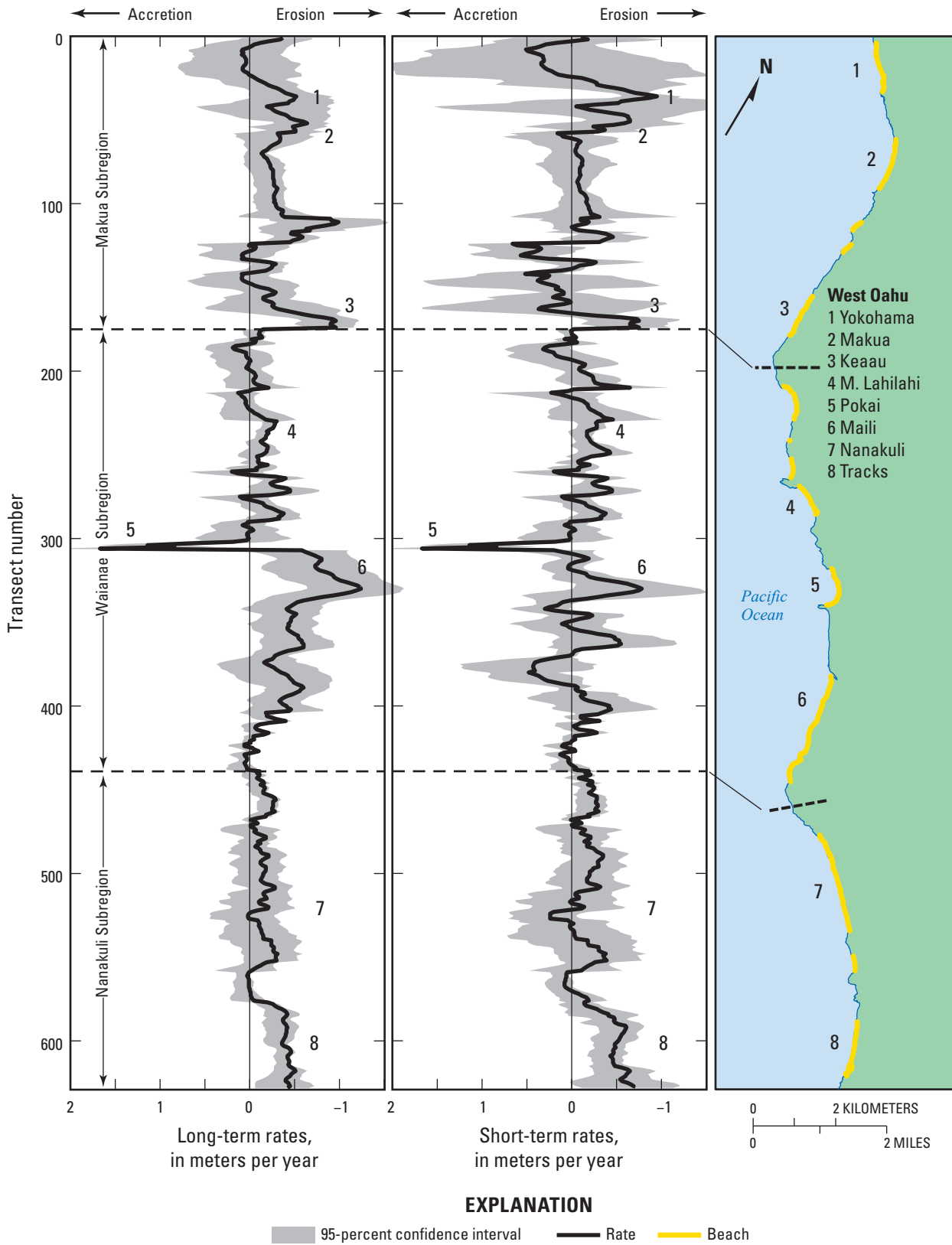
Figure 30. Long-term (all available years) and short-term (1940s to present) shoreline change rates, West Oahu. (Location shown in figure 22)
