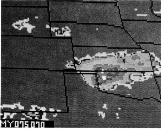
Figure 7. GOES-West, IR satellite photo from 0700 GMT on 7 May 1985 showing developing MCC over the eastern TX panhandle and western OK.
