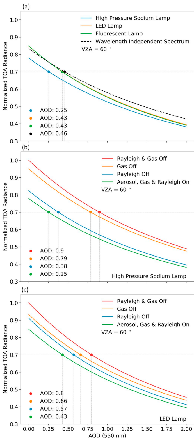
Fig. 7. (a) I_{norm} as a function of AOD for different surface illumination spectra. (b) and (c) are similar as (a) but respectively for surface illumination spectra of HPS only and LED only with different treatments of turning on and off gas absorption and Rayleigh scattering.
