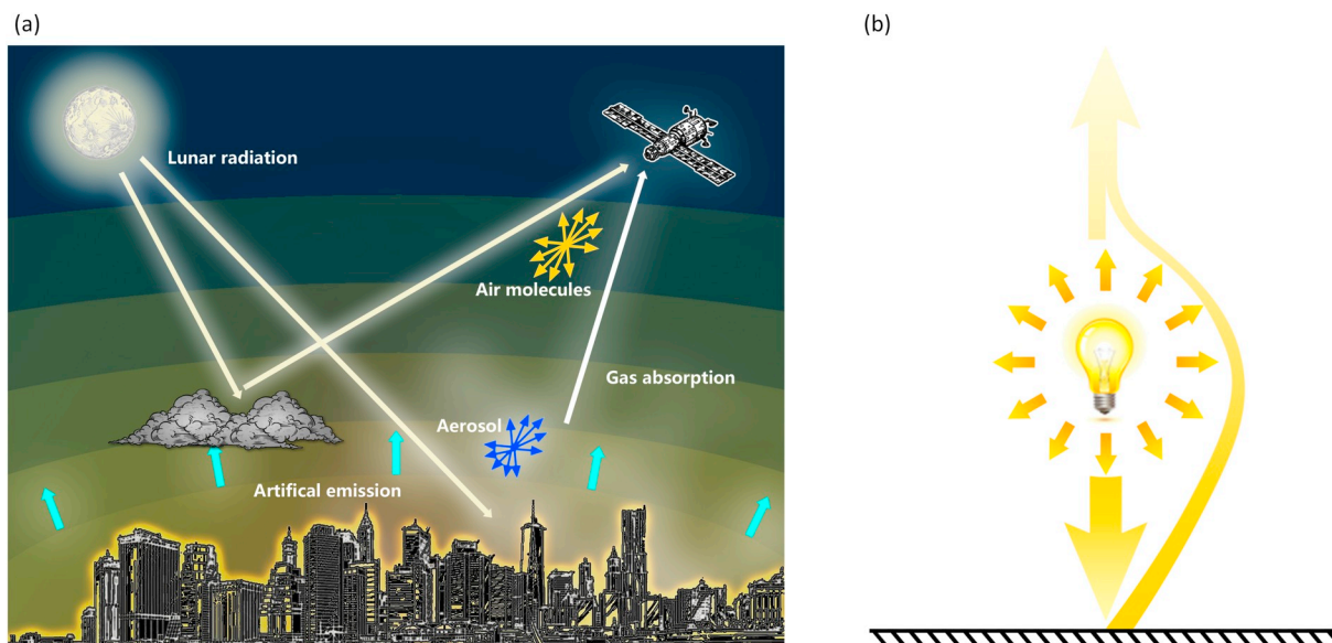
Fig. 1. (a) Key components of nighttime radiative transfer in cloud-free conditions. (b) Representation of surface bulb illumination and its interaction with surface in the model development. Please see text for details.
