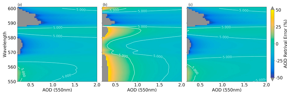
Fig. 8. Relative bias (in %) in AOD as a function of the true AOD (x-axis) and the narrow-band wavelengths (y-axis) used for the retrieval from DNB radiance for the surfaces illuminated by (a) LED, (b) HPS, and (c) FL, respectively. Regions with bias > 50% is shown as grey.
