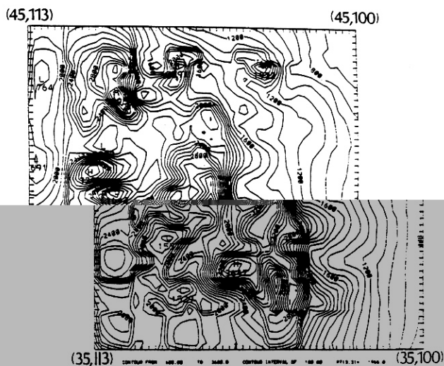
Figure 10: Model topography (grids 2 and 3) for simulations of the 30-31 March 1988 storm. Elevations are in m.
