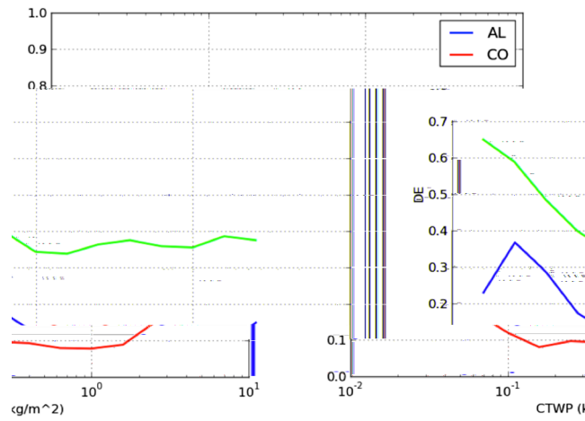
Figure 12. The detection efficiency versus CWP for Alabama (blue) and Colorado (red).
