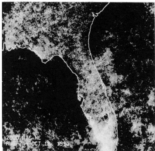
Fig. 3: Cloud frequency composites at 15 (a), 18 (b) and 20 UTC (c) for NE flow days.
