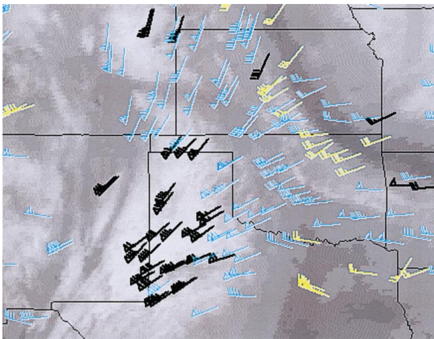
FIG. 11. GOES-derived winds at 1800 UTC 3 May 1999. Black bars are in the 100–250-hPa layer, cyan bars in the 251–350-hPa layer, and yellow bars are in the 351–500-hPa layer. Wind speeds are in knots.
